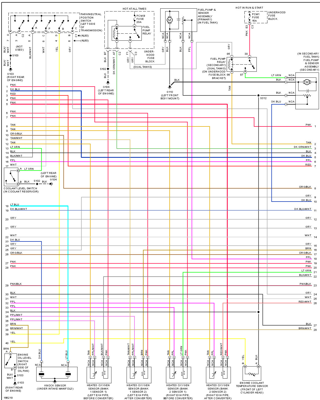
Fig. 21: 6.0L VIN U, Engine Performance Circuit (2 of 5)
