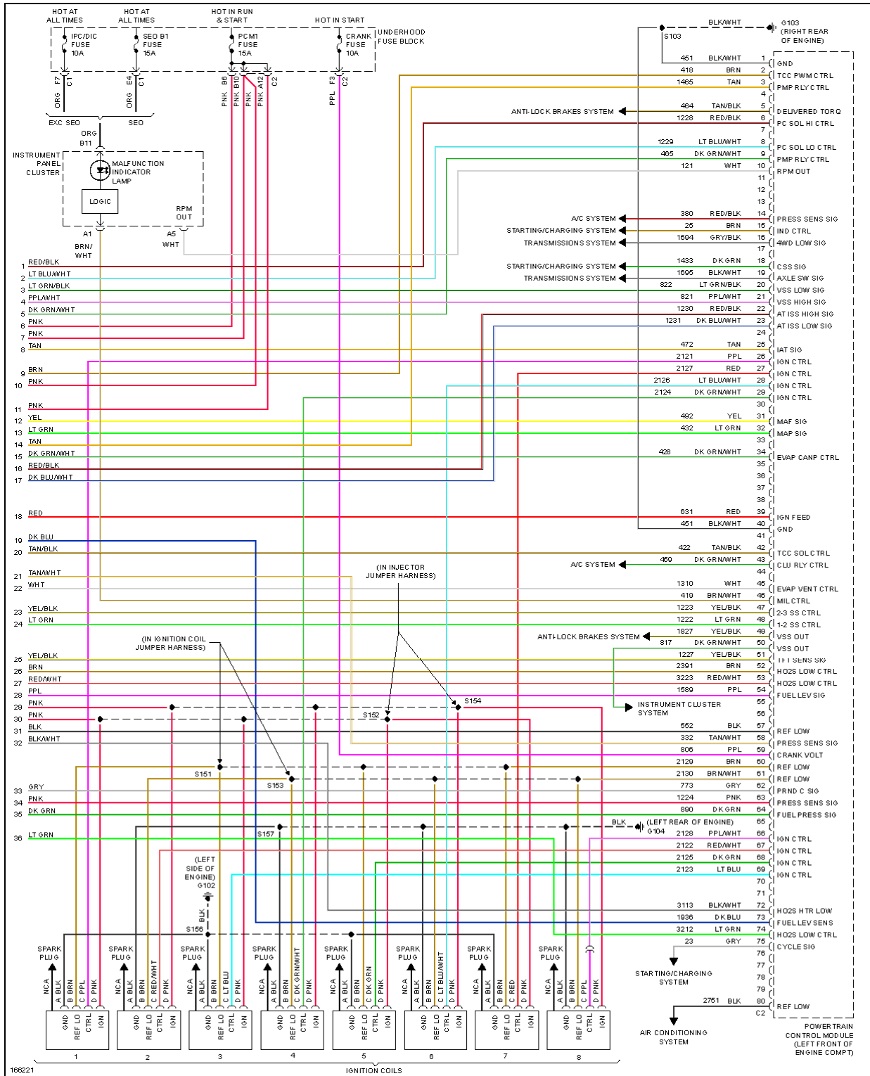
Fig. 24: 6.0L VIN U, Engine Performance Circuit (5 of 5)
