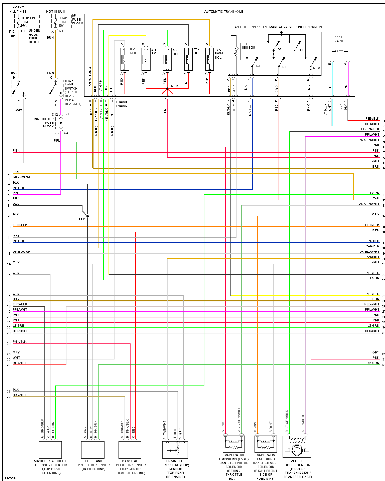
Fig. 44: 6.0L VIN U, Engine Performance Circuit (3 of 5)
