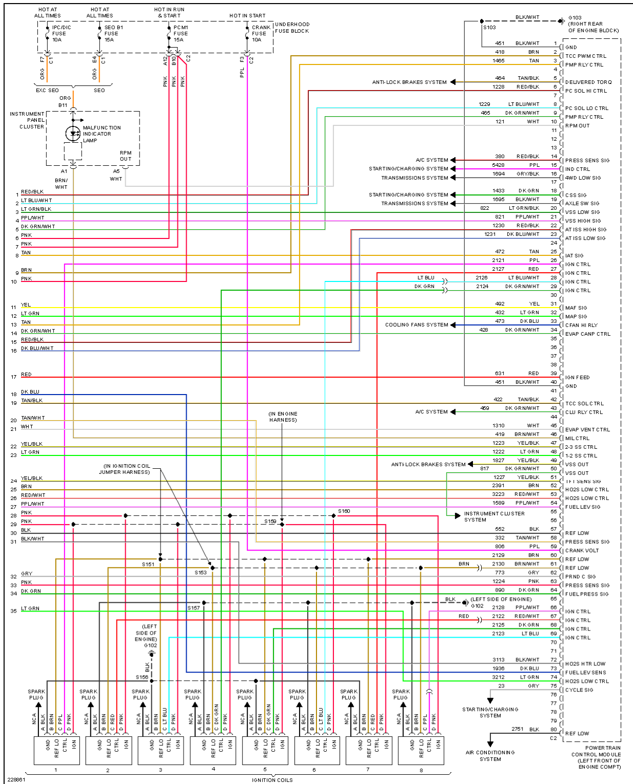
Fig. 46: 6.0L VIN U, Engine Performance Circuit (5 of 5)
