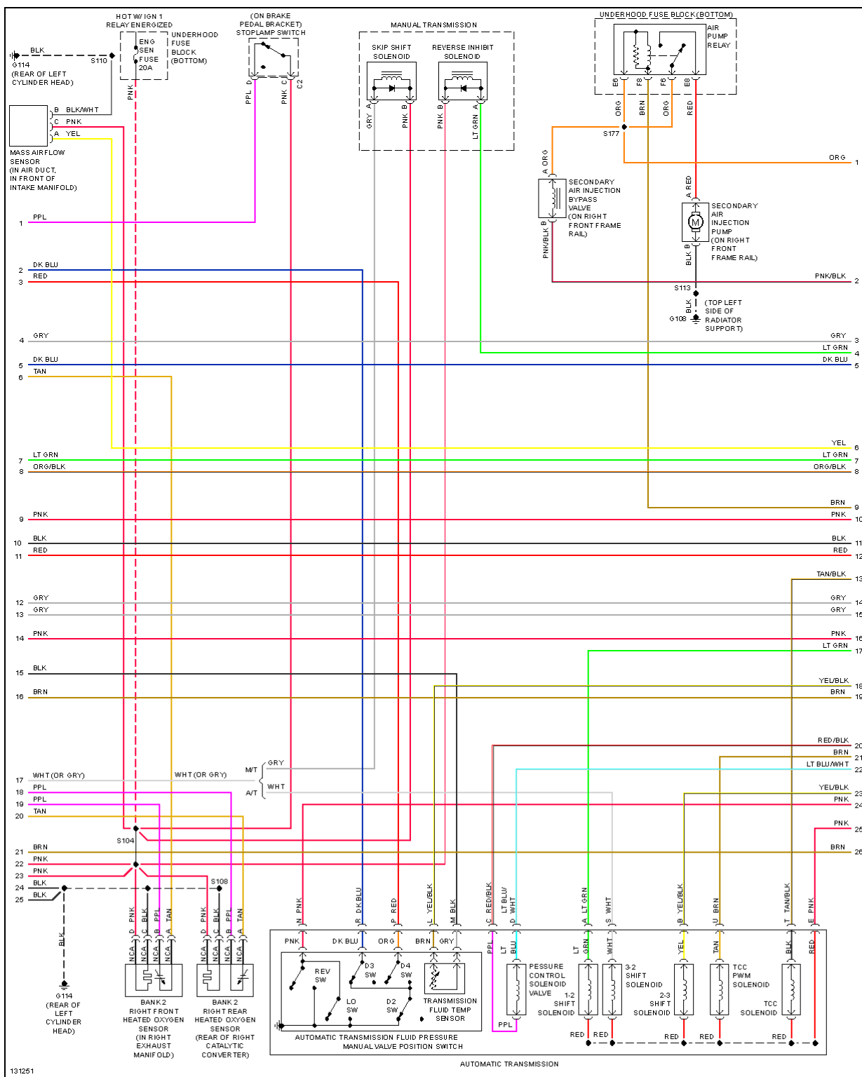
Fig. 21: 5.7L VIN G, Engine Performance Circuits (2 of 4)
