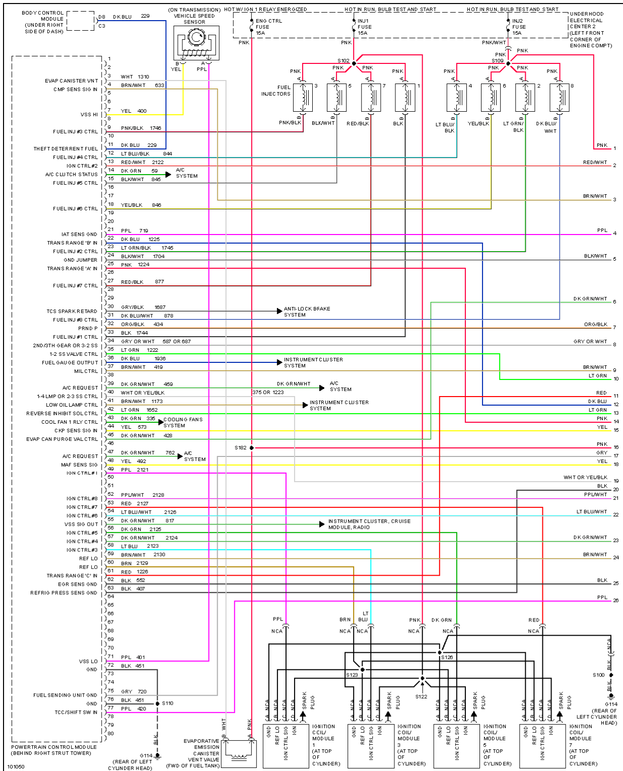
Fig. 15: 5.7L (VIN G), Engine Performance Circuits (1 of 4)
