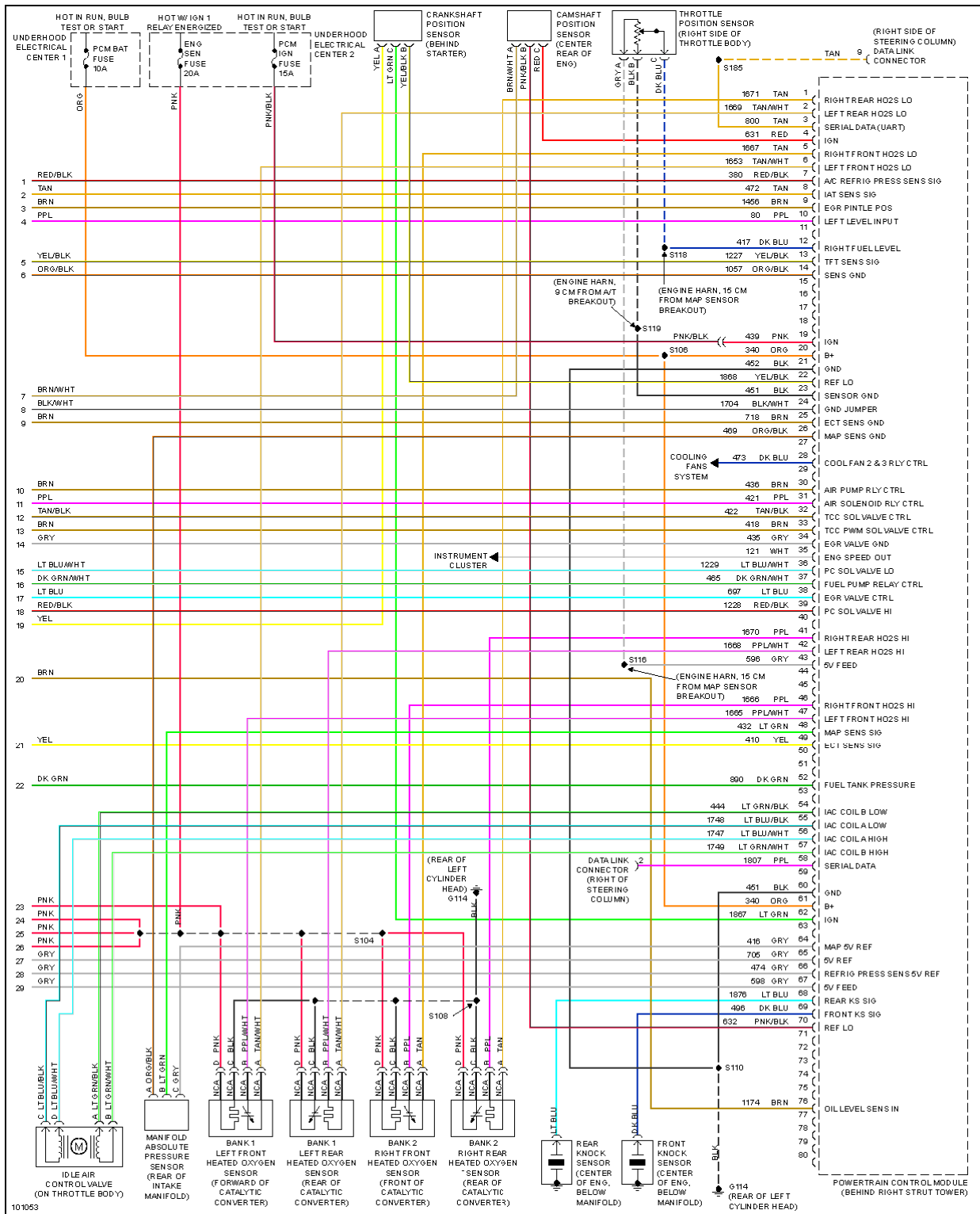
Fig. 18: 5.7L (VIN G), Engine Performance Circuits (4 of 4)
