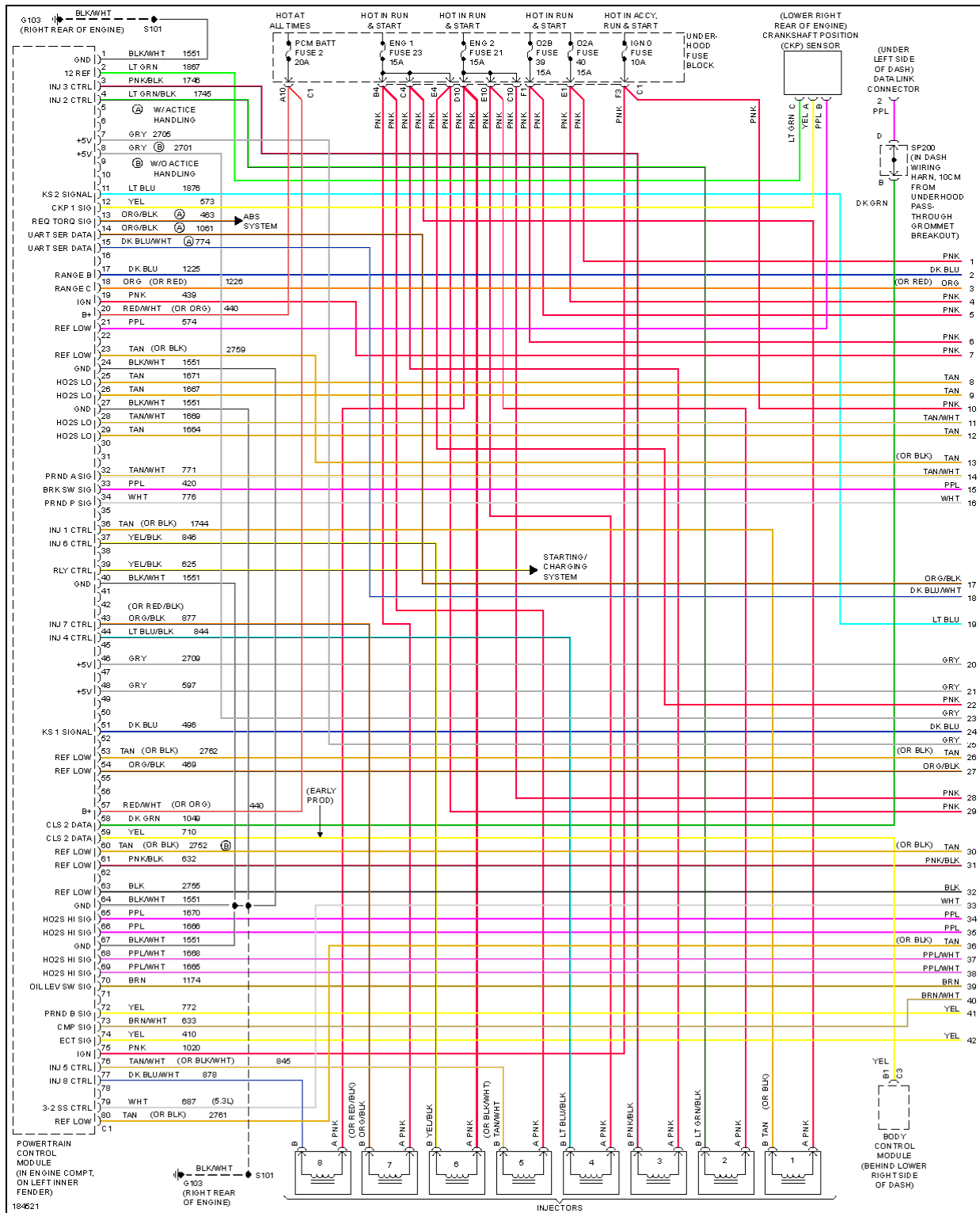
Fig. 37: 6.0L VIN U, Engine Performance Circuit (1 of 5)
