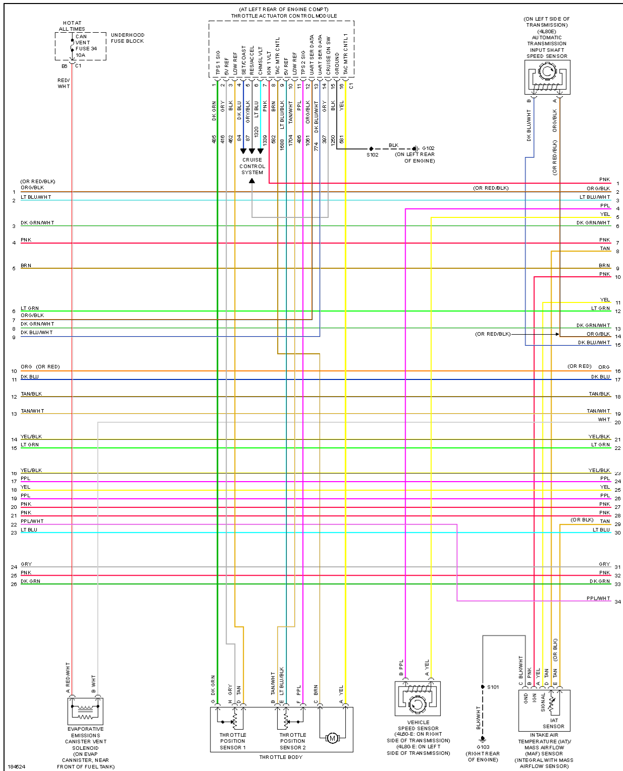
Fig. 40: 6.0L VIN U, Engine Performance Circuit (4 of 5)
