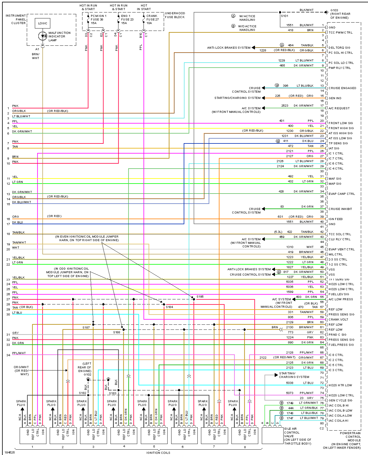
Fig. 41: 6.0L VIN U, Engine Performance Circuit (5 of 5)
