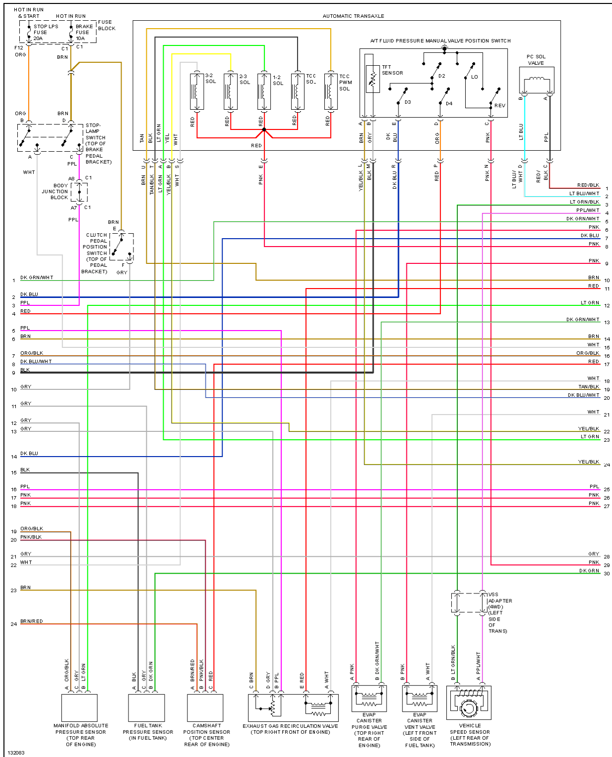
Fig. 35: 5.3L VIN T, Engine Performance Circuits, W/ Delphi HO2S (3 of 5)
