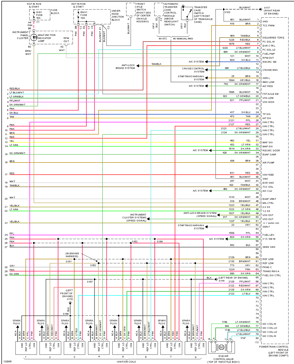
Fig. 37: 5.3L VIN T, Engine Performance Circuits, W/ Delphi HO2S (5 of 5)
