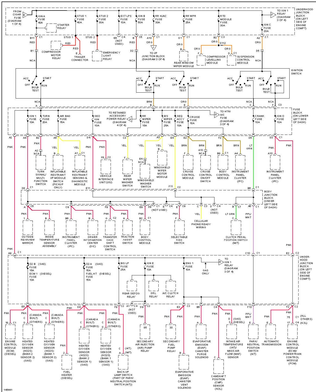
Fig. 64: Power Distribution Circuit (2 of 4)
