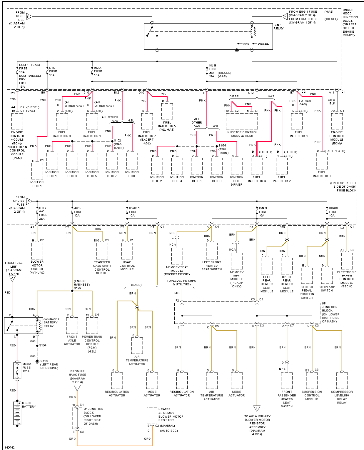
Fig. 65: Power Distribution Circuit (3 of 4)
