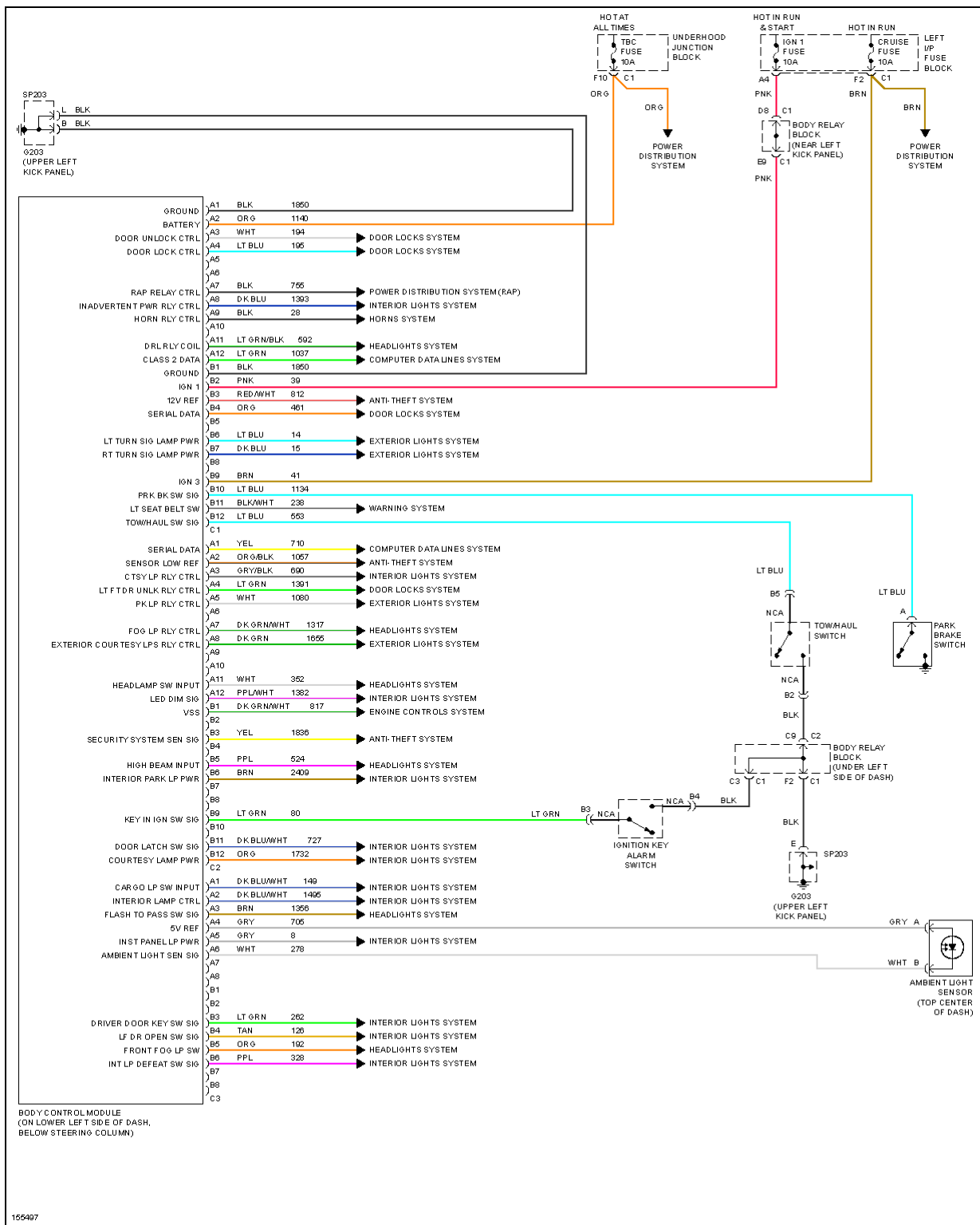
Fig. 11: Body Computer Circuits
