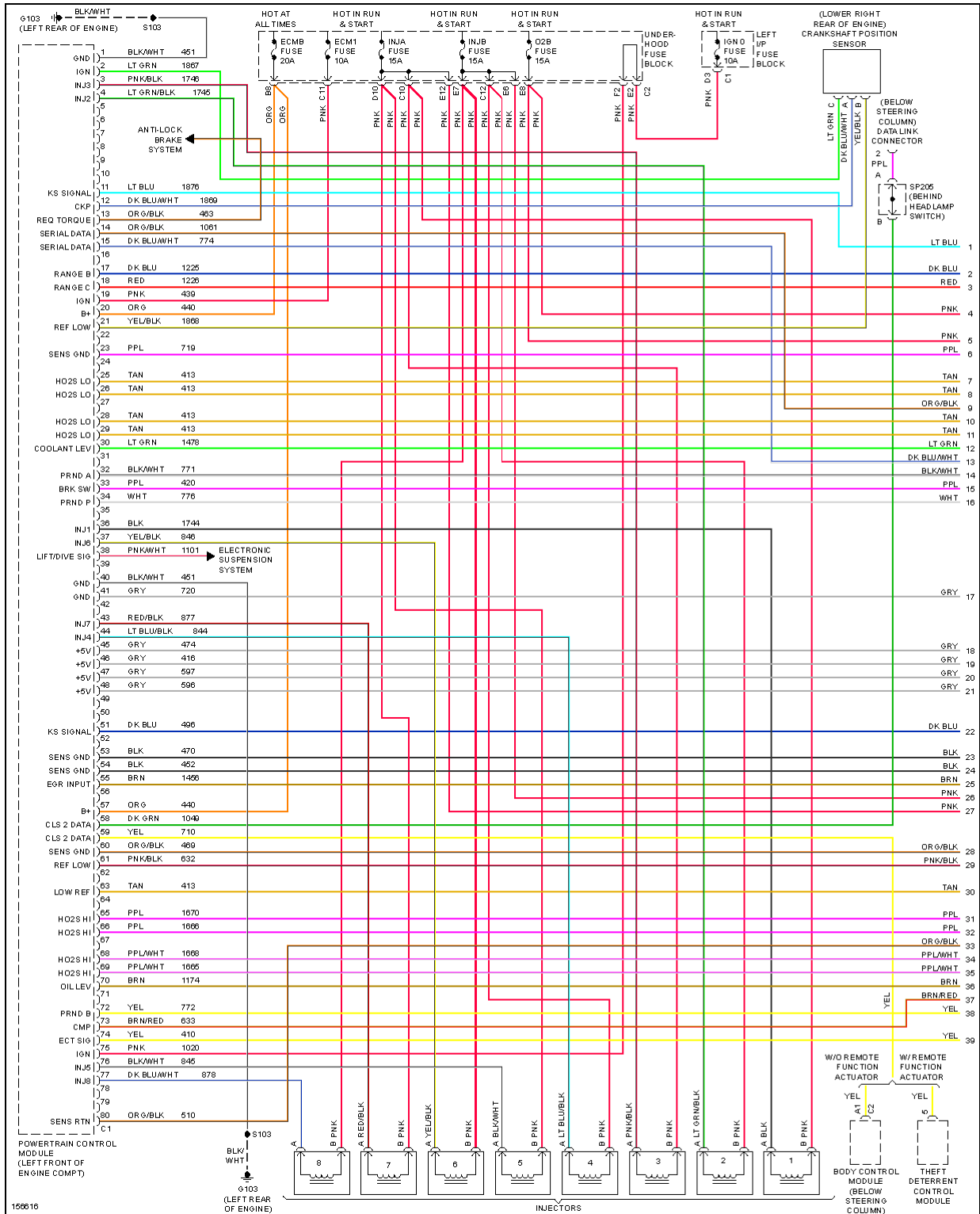
Fig. 25: 6.0L VIN U, Engine Performance Circuits, W/ Isolated Grounded HO2S Sensors (1 of 5)
