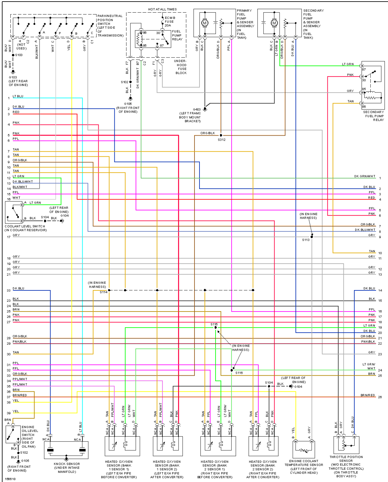
Fig. 26: 6.0L VIN U, Engine Performance Circuits, W/ Isolated Grounded HO2S Sensors (2 of 5)
