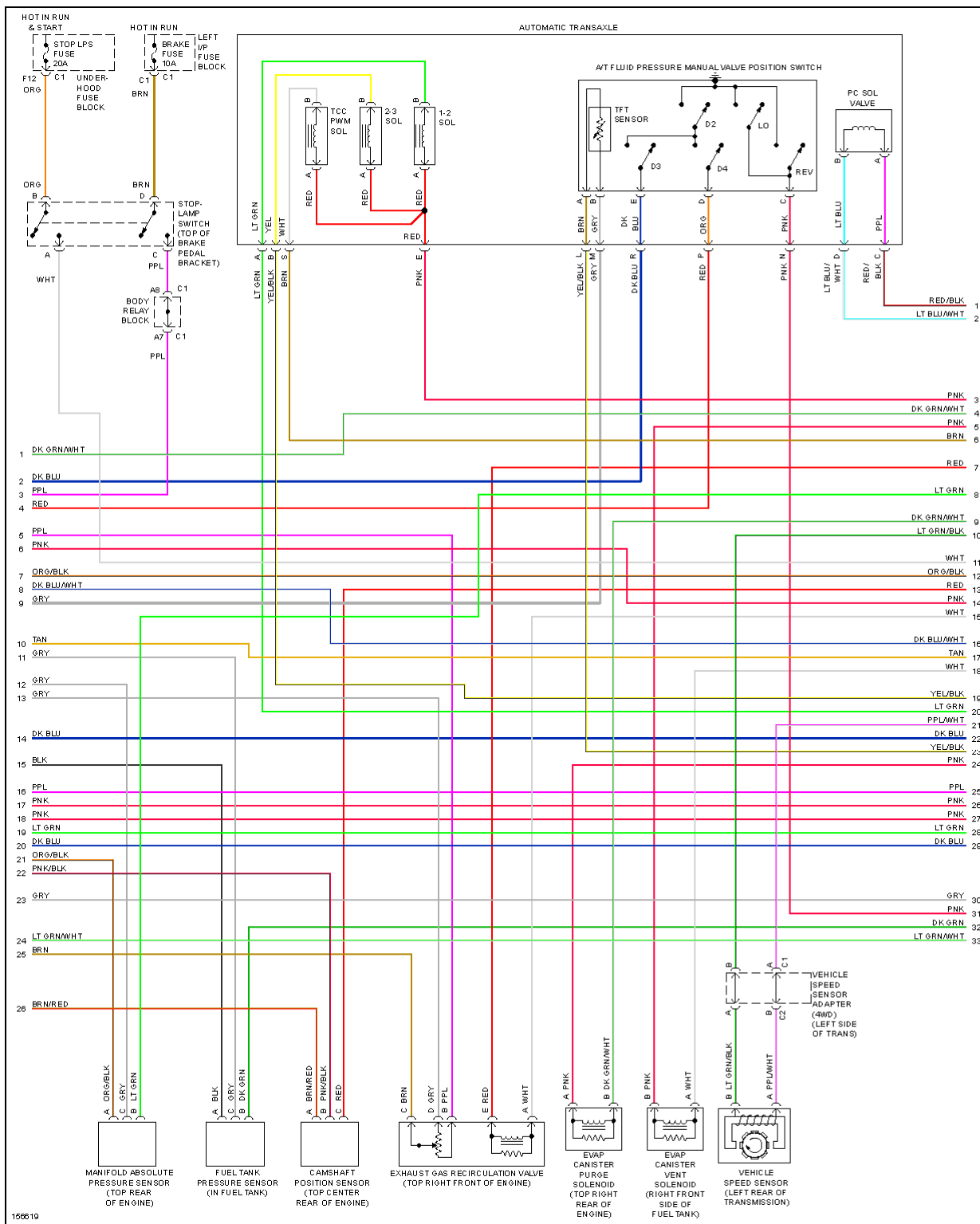
Fig. 27: 6.0L VIN U, Engine Performance Circuits, W/ Isolated Grounded HO2S Sensors (3 of 5)
