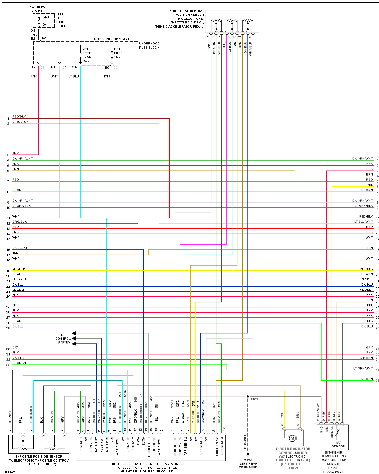
Fig. 28: 6.0L VIN U, Engine Performance Circuits, W/ Isolated Grounded HO2S Sensors (4 of 5)
