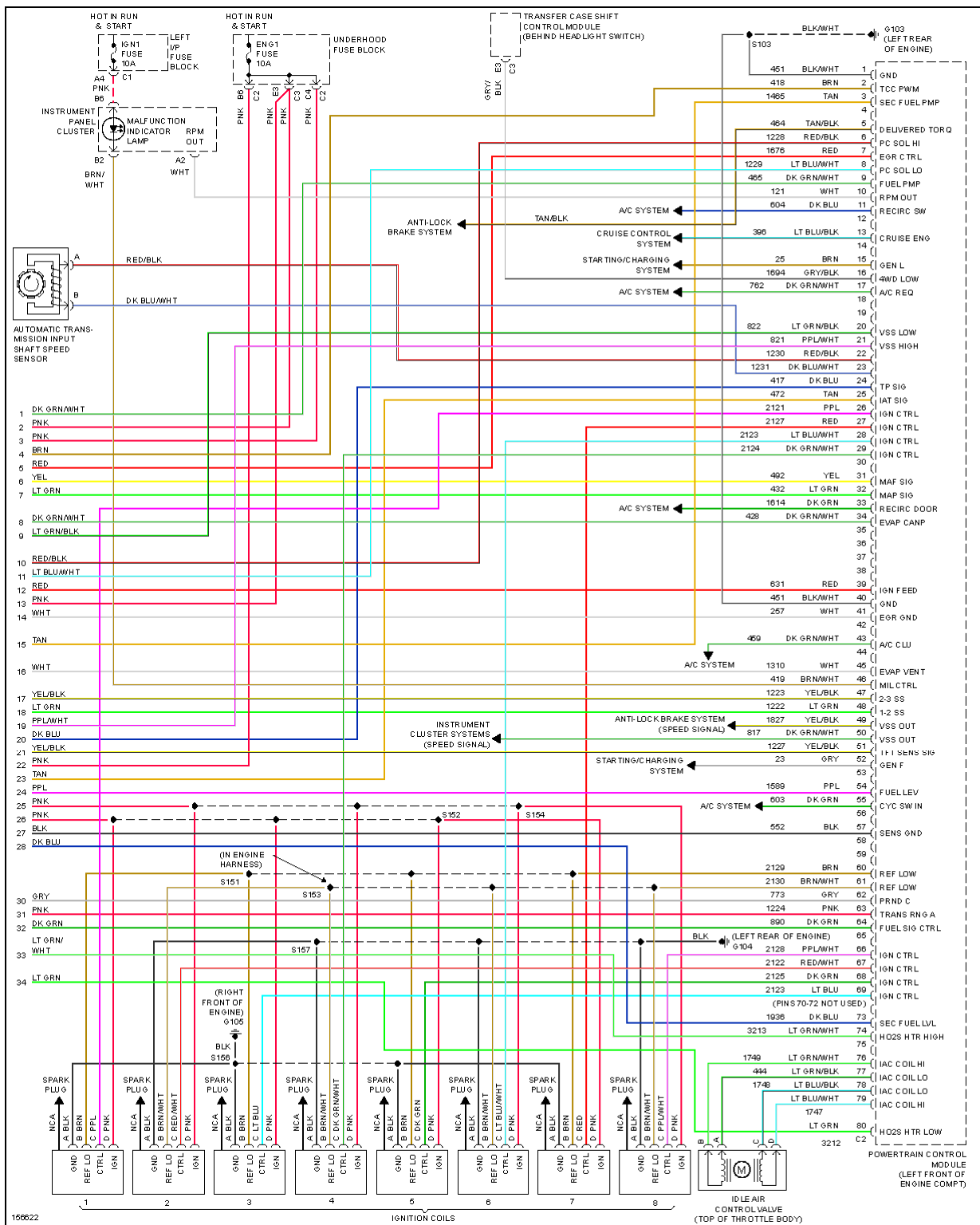
Fig. 29: 6.0L VIN U, Engine Performance Circuits, W/ Isolated Grounded HO2S Sensors (5 of 5)
