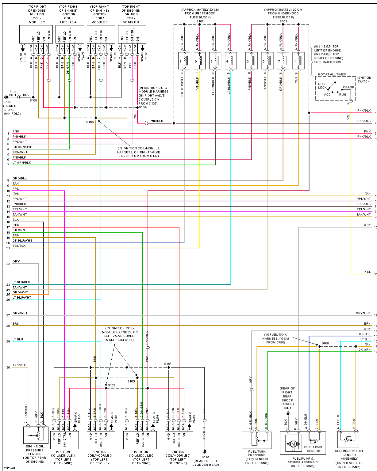
Fig. 27: 6.0L VIN U, Engine Performance Circuit (2 of 5)
