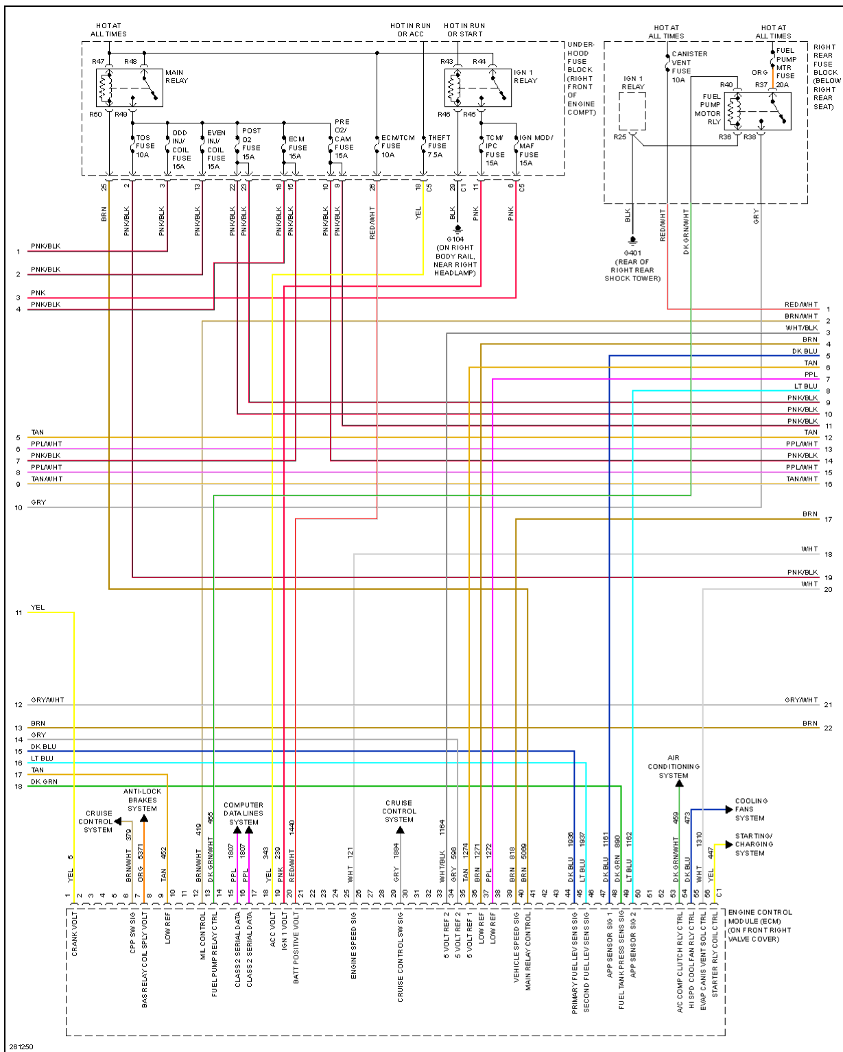
Fig. 28: 6.0L VIN U, Engine Performance Circuit (3 of 5)
