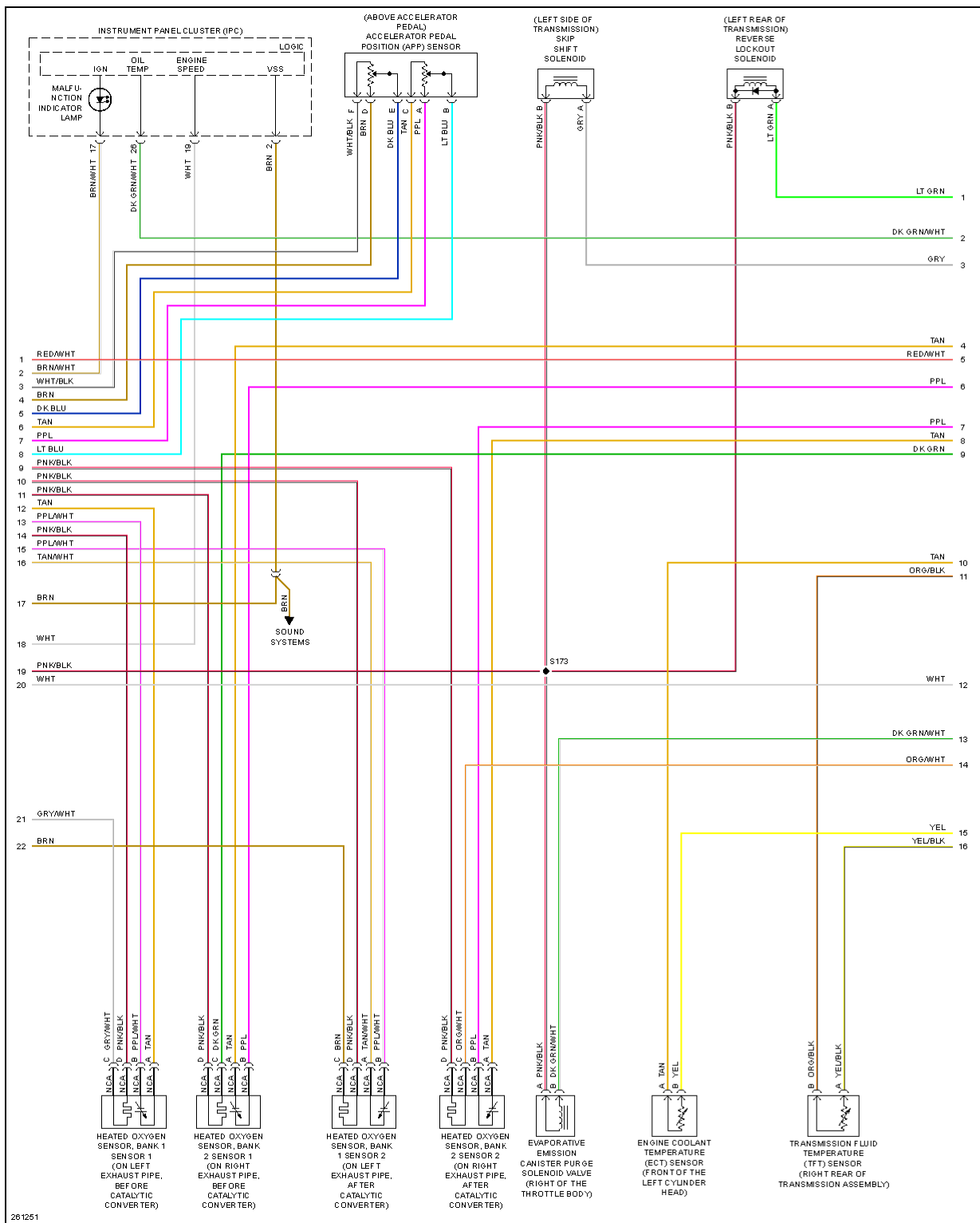
Fig. 29: 6.0L VIN U, Engine Performance Circuit (4 of 5)
