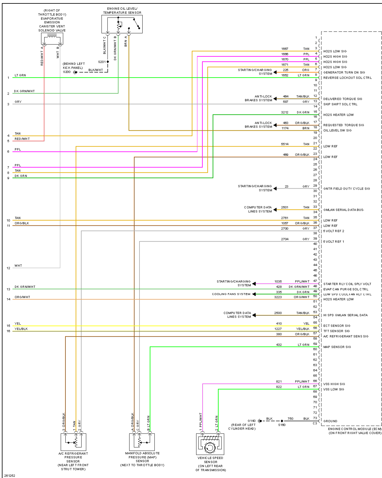
Fig. 30: 6.0L VIN U, Engine Performance Circuit (5 of 5)
