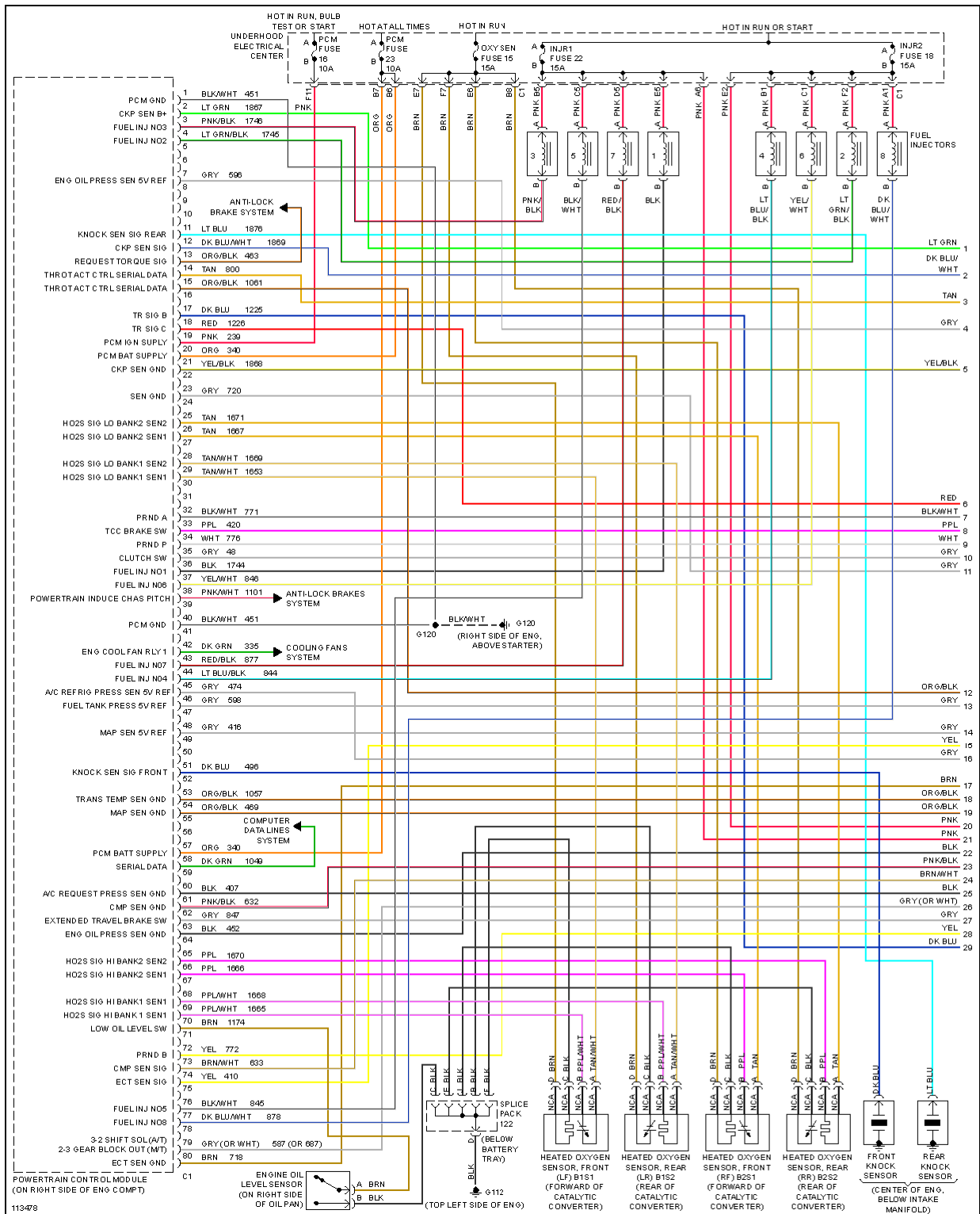
Fig. 14: 5.7L VIN G, Engine Performance Circuits (1 of 4)
