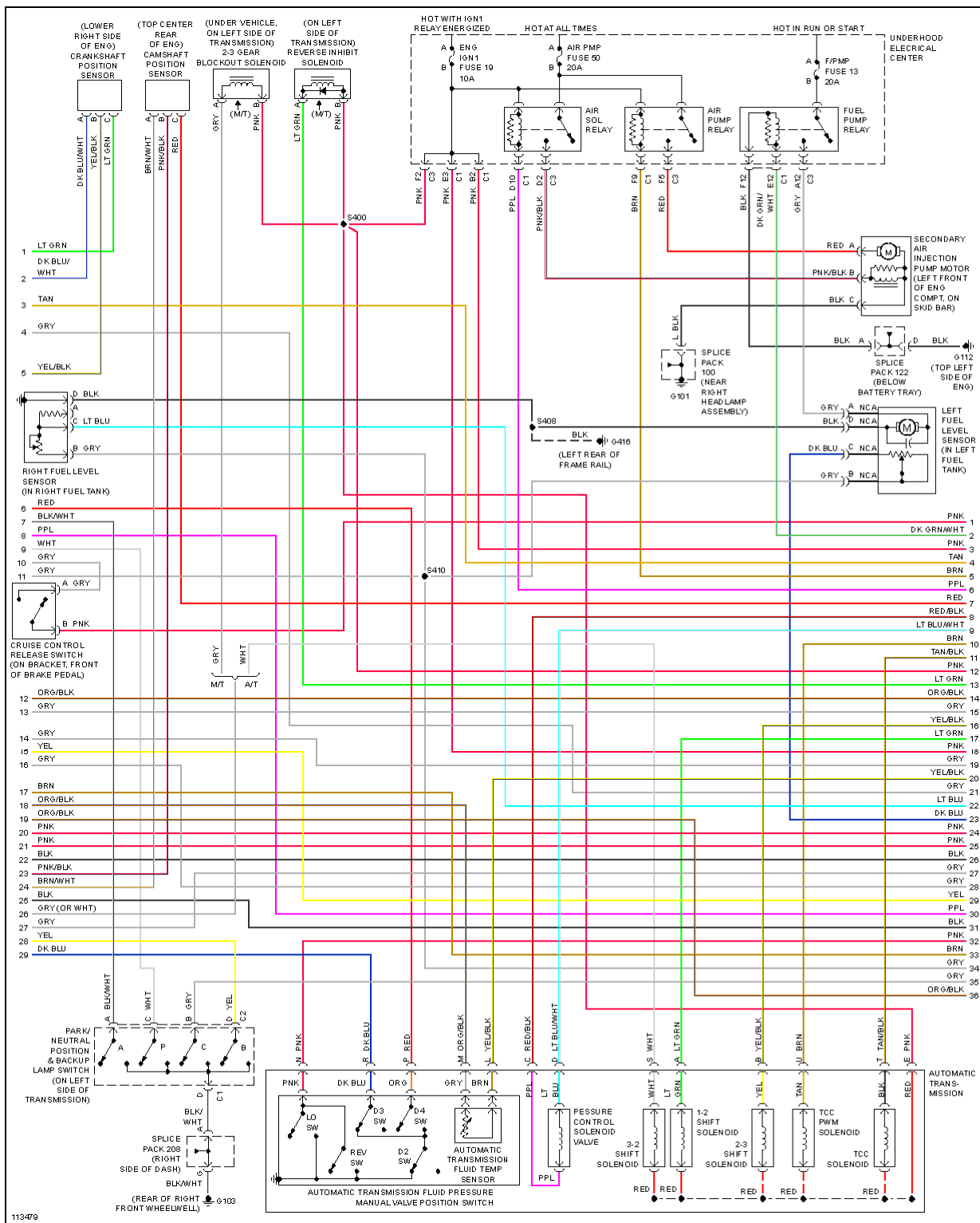
Fig. 15: 5.7L VIN G, Engine Performance Circuits (2 of 4)
