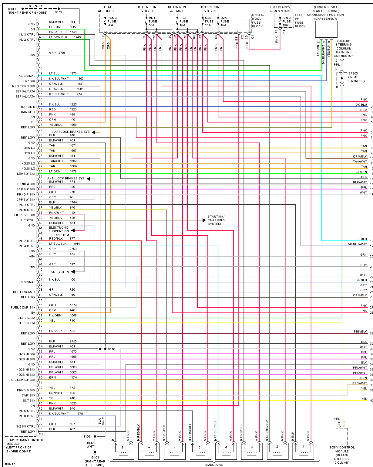
Fig. 21: 6.0L VIN U, Engine Performance Circuit (1 of 5)
