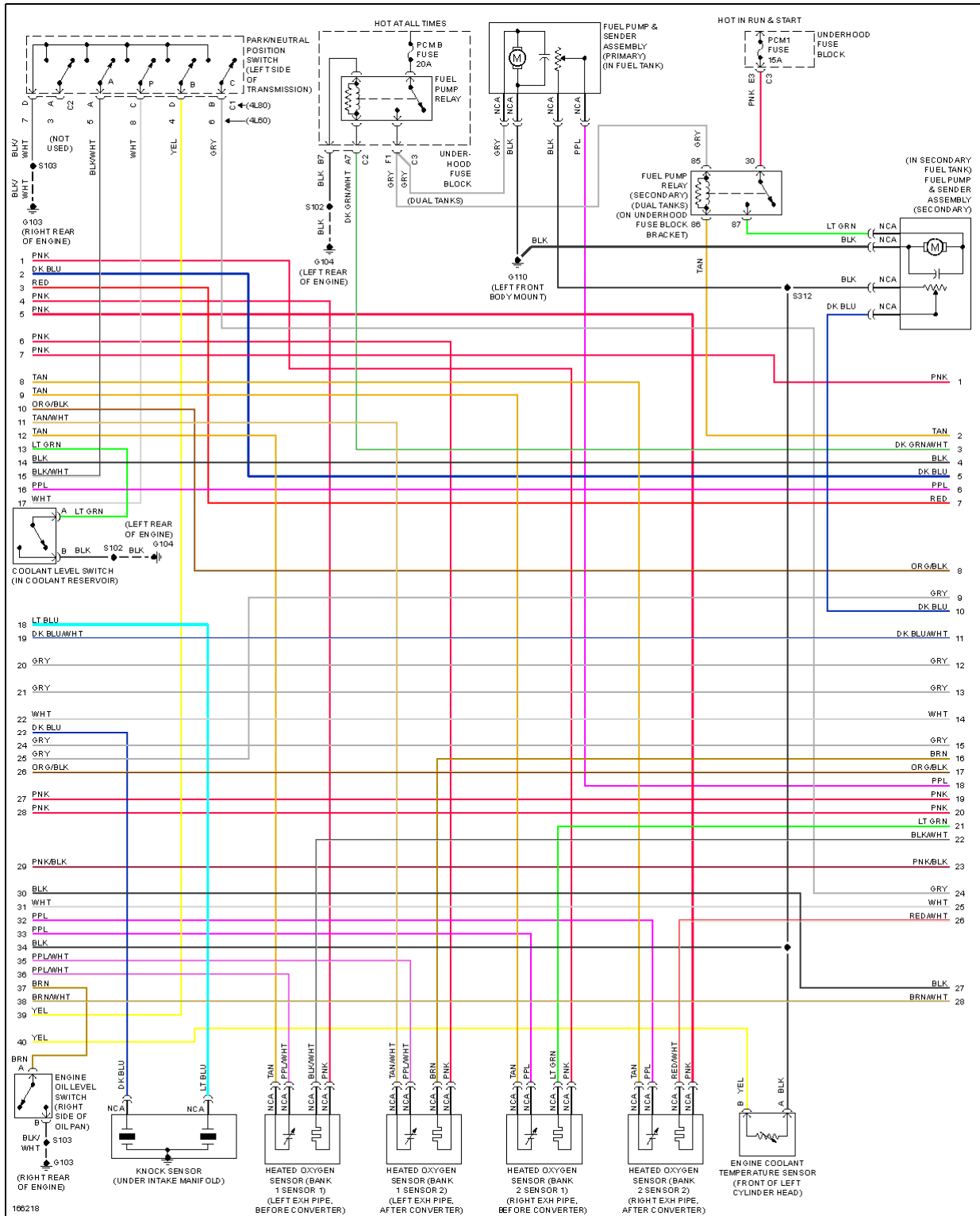
Fig. 22: 6.0L VIN U, Engine Performance Circuit (2 of 5)
