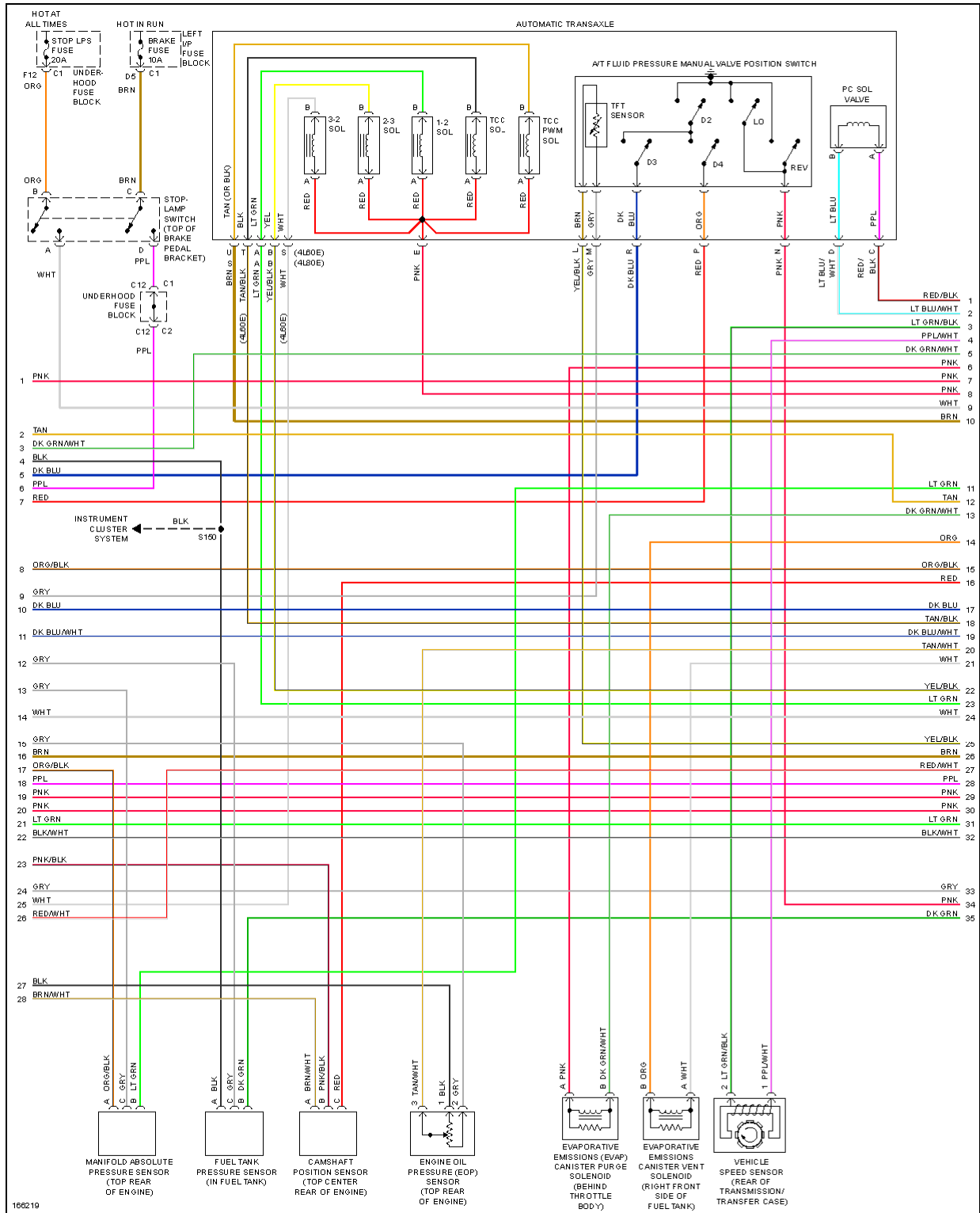
Fig. 23: 6.0L VIN U, Engine Performance Circuit (3 of 5)
