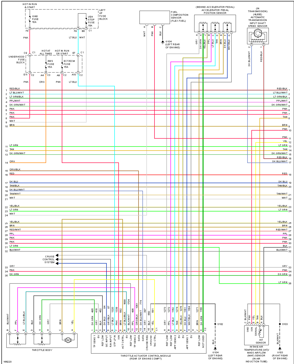
Fig. 24: 6.0L VIN U, Engine Performance Circuit (4 of 5)
