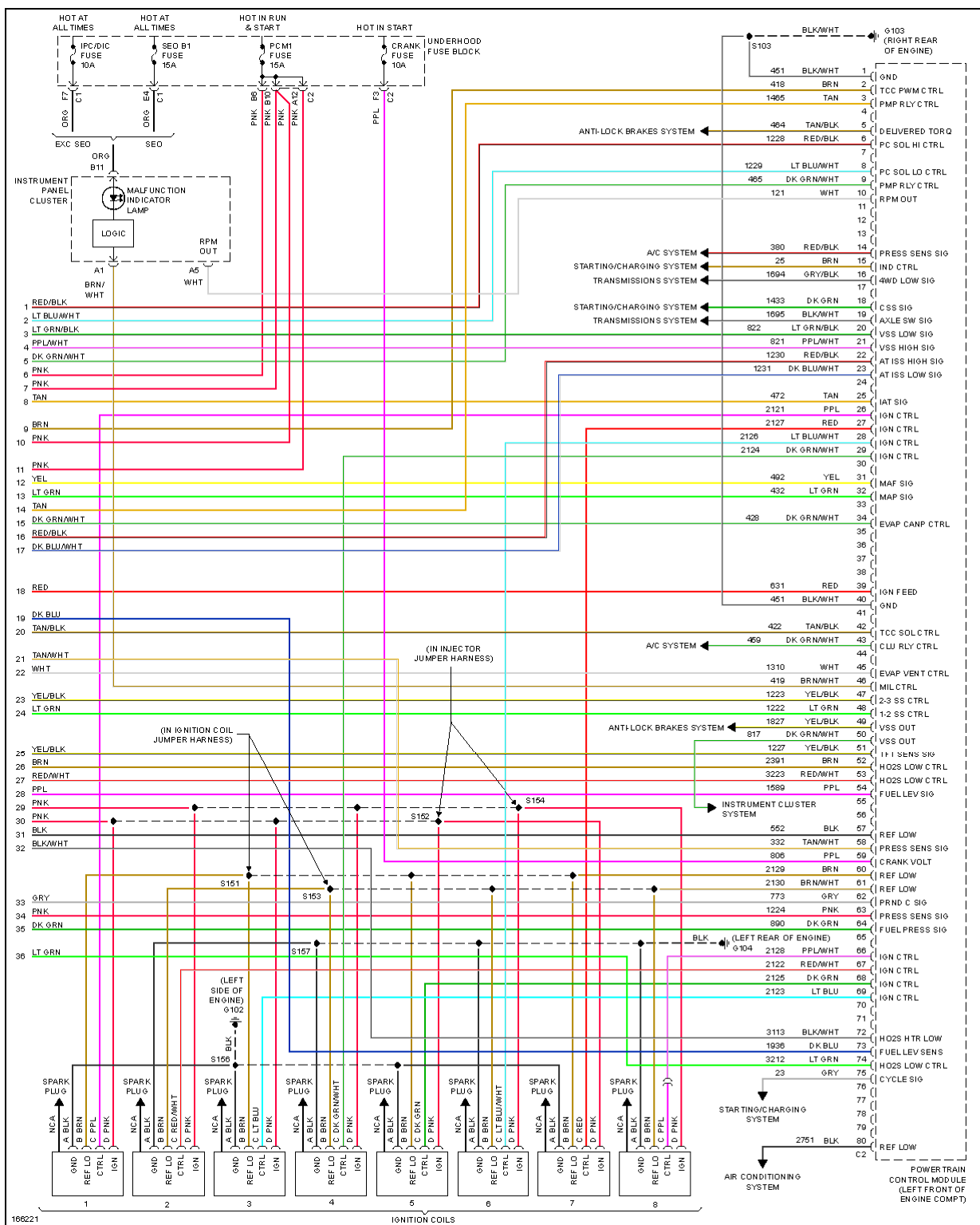
Fig. 25: 6.0L VIN U, Engine Performance Circuit (5 of 5)
