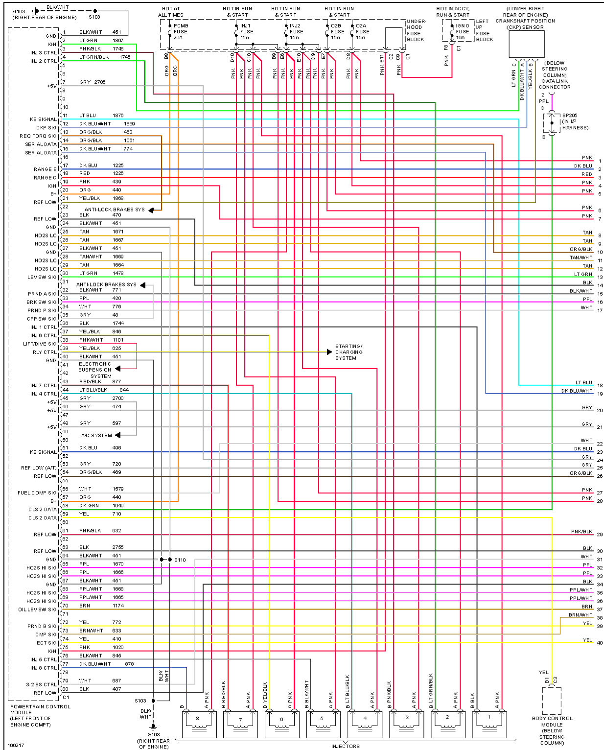
Fig. 37: 5.3L VIN Z, Engine Performance Circuit (1 of 5)
