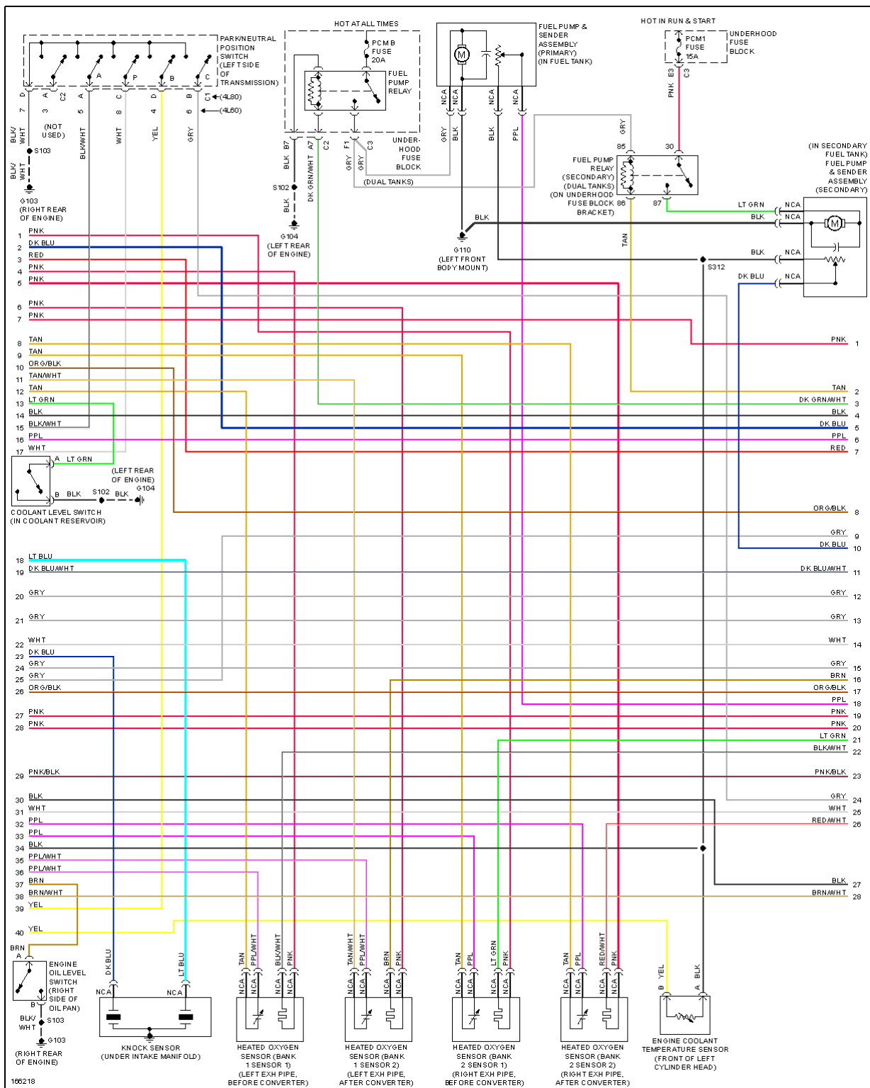
Fig. 38: 5.3L VIN Z, Engine Performance Circuit (2 of 5)
