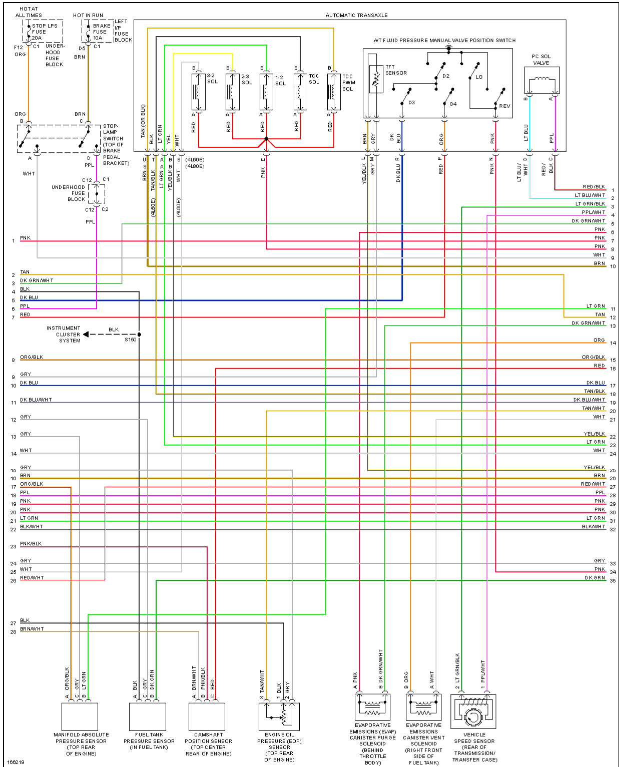
Fig. 39: 5.3L VIN Z, Engine Performance Circuit (3 of 5)
