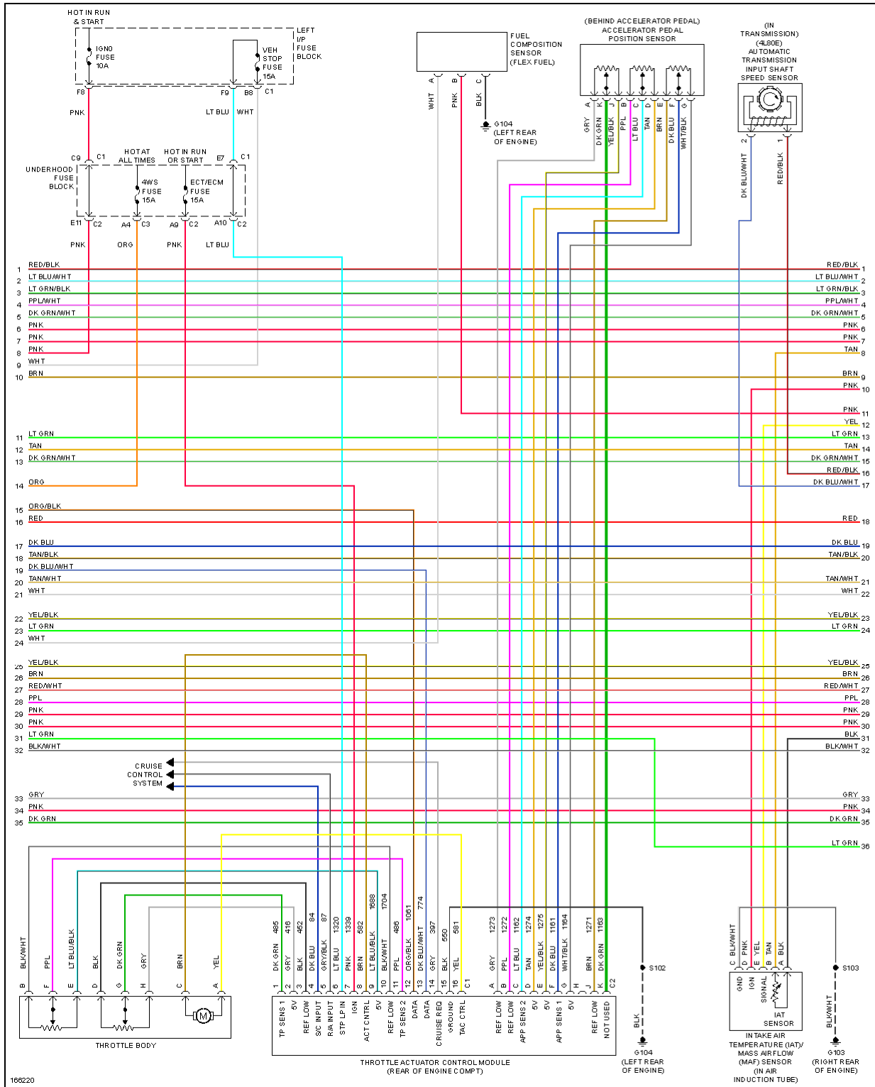
Fig. 40: 5.3L VIN Z, Engine Performance Circuit (4 of 5)
