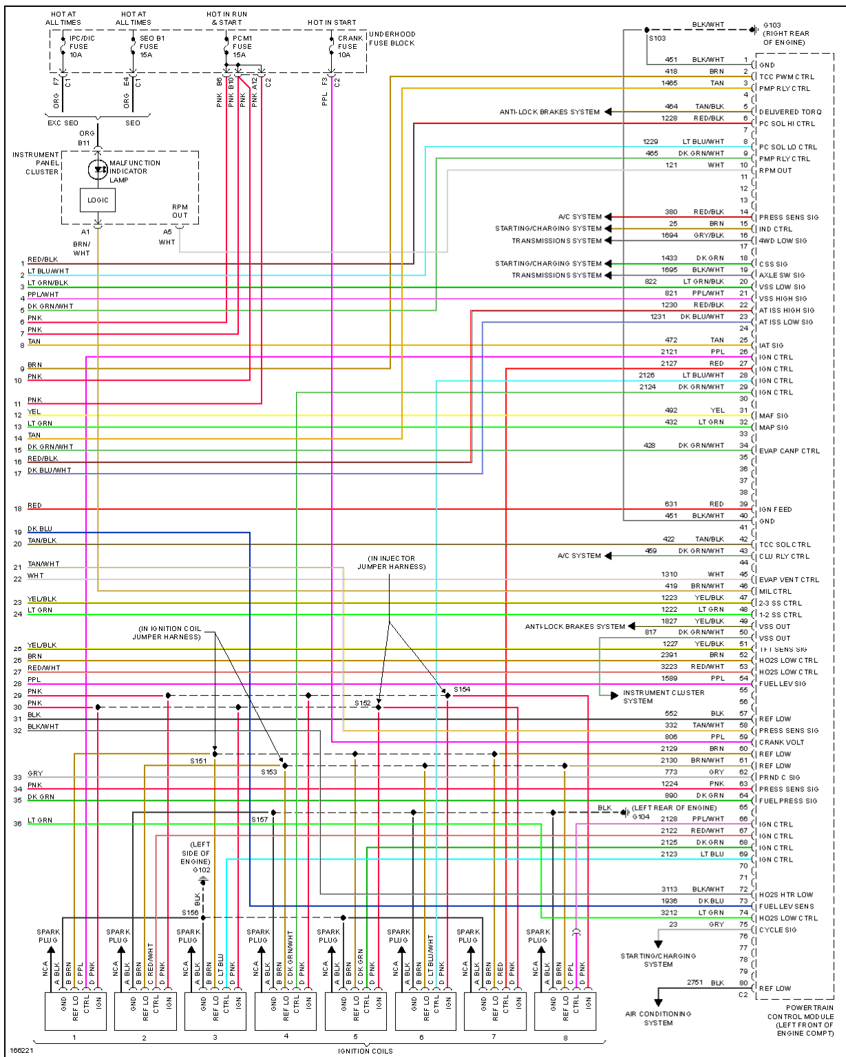
Fig. 41: 5.3L VIN Z, Engine Performance Circuit (5 of 5)
