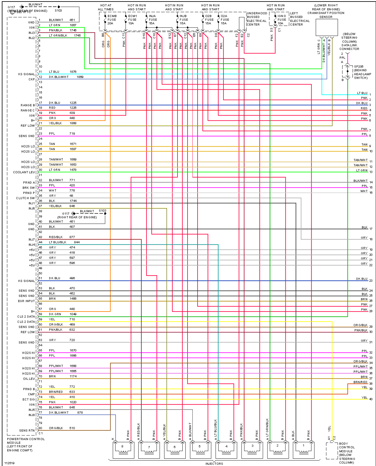
Fig. 25: 6.0L VIN U, Engine Performance Circuits (1 of 4)
