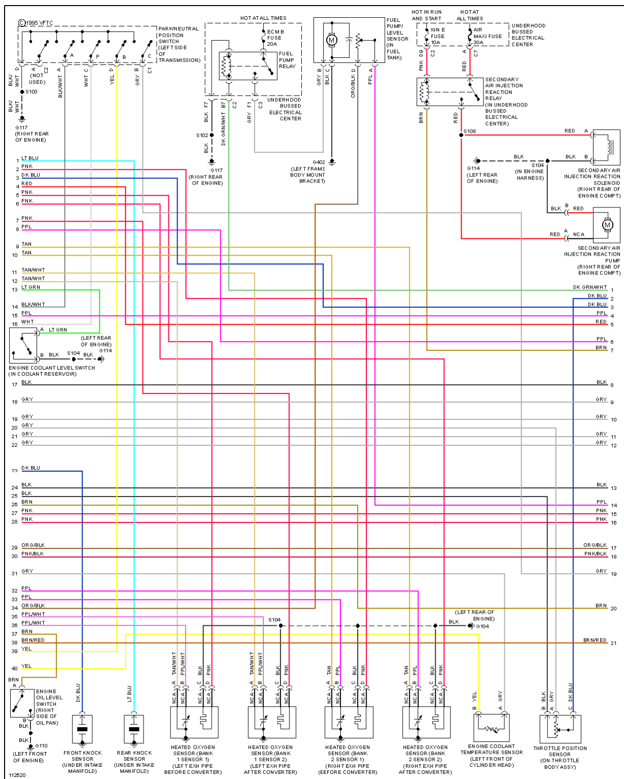
Fig. 26: 6.0L VIN U, Engine Performance Circuits (2 of 4)
