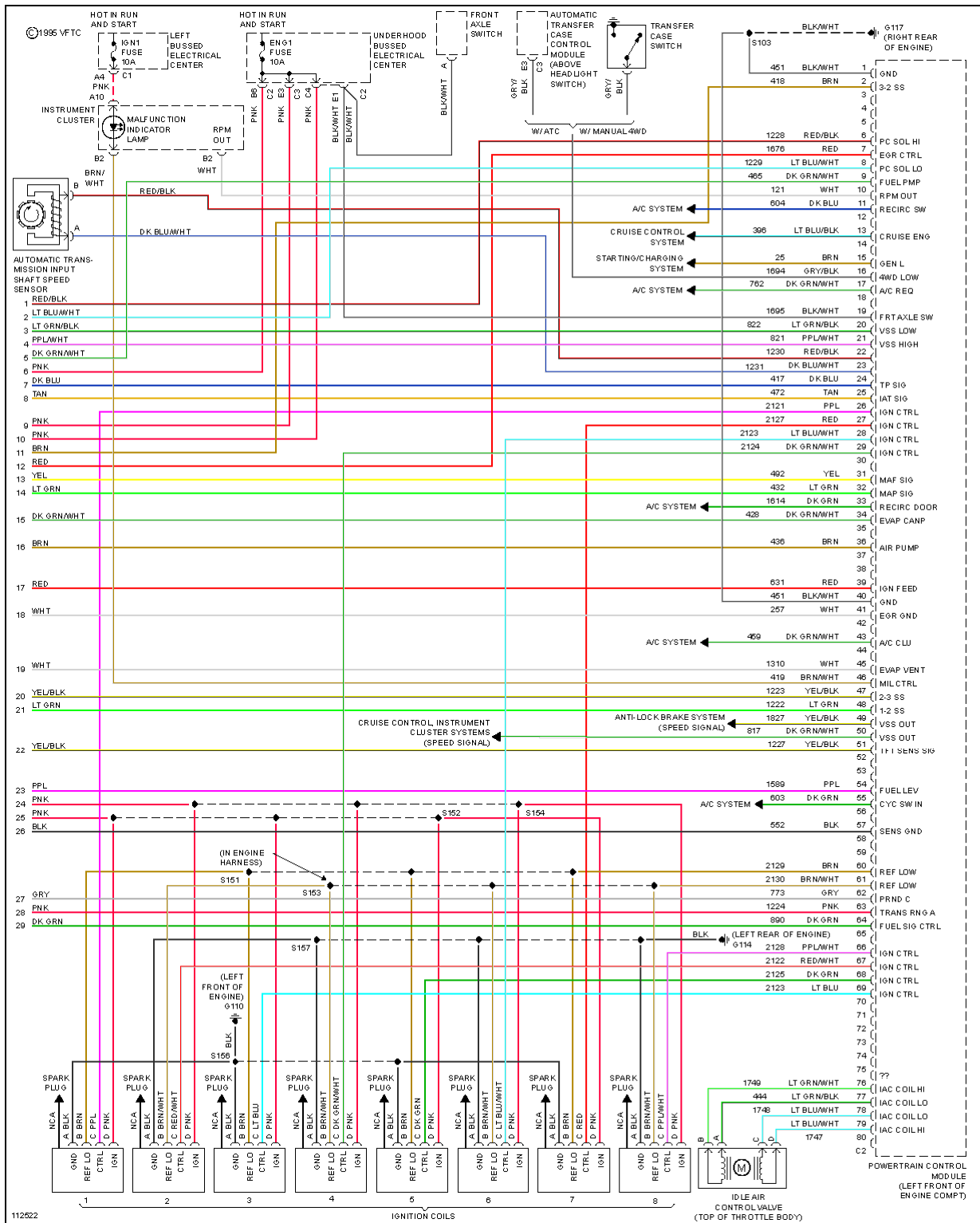
Fig. 28: 6.0L VIN U, Engine Performance Circuits (4 of 4)
