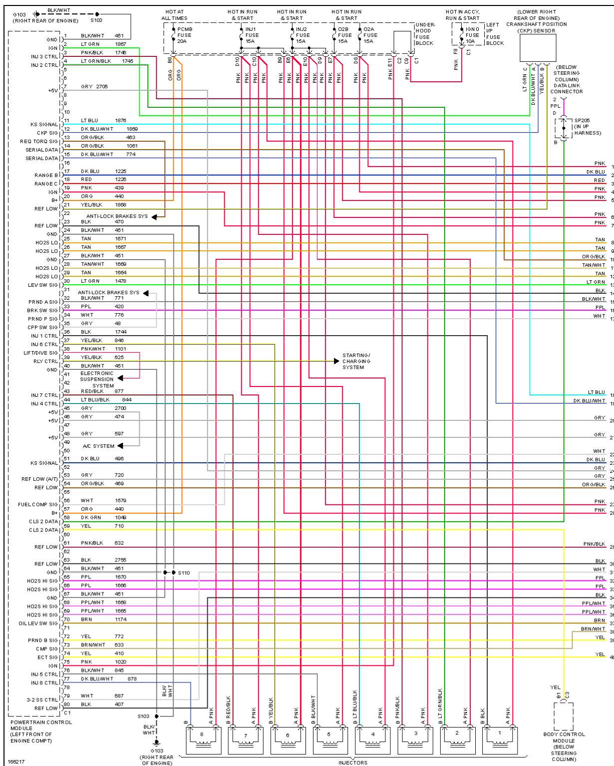
Fig. 20: 6.0L VIN U, Engine Performance Circuit (1 of 5)
