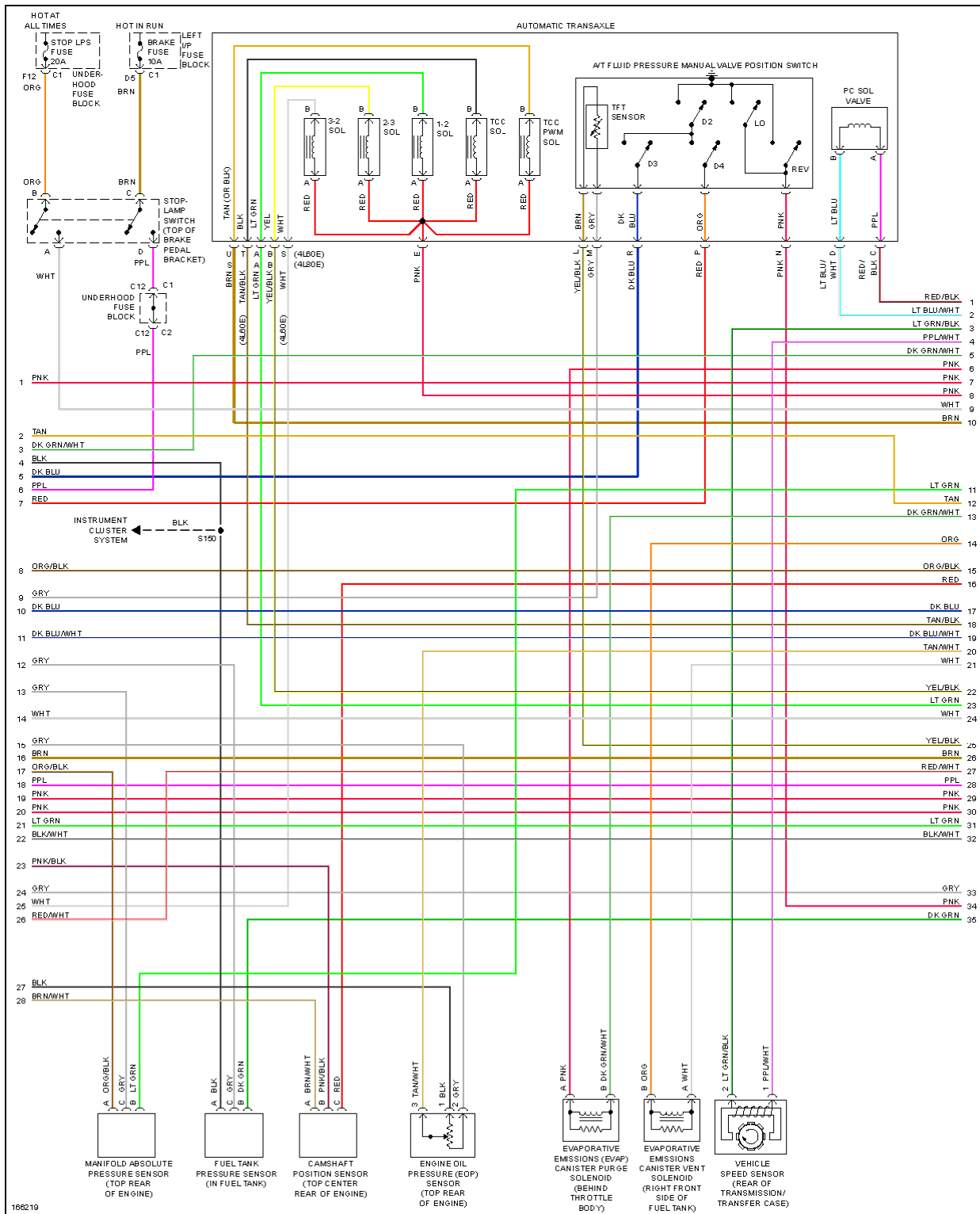
Fig. 22: 6.0L VIN U, Engine Performance Circuit (3 of 5)
