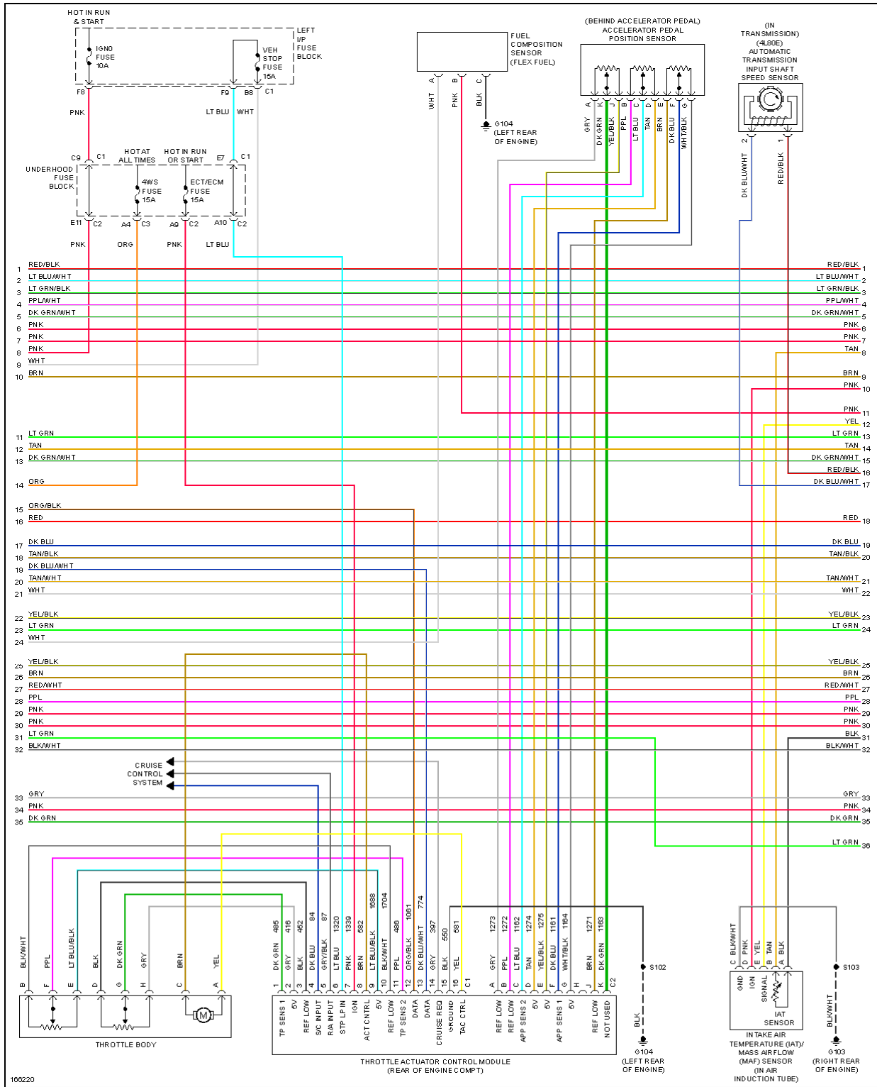
Fig. 23: 6.0L VIN U, Engine Performance Circuit (4 of 5)
