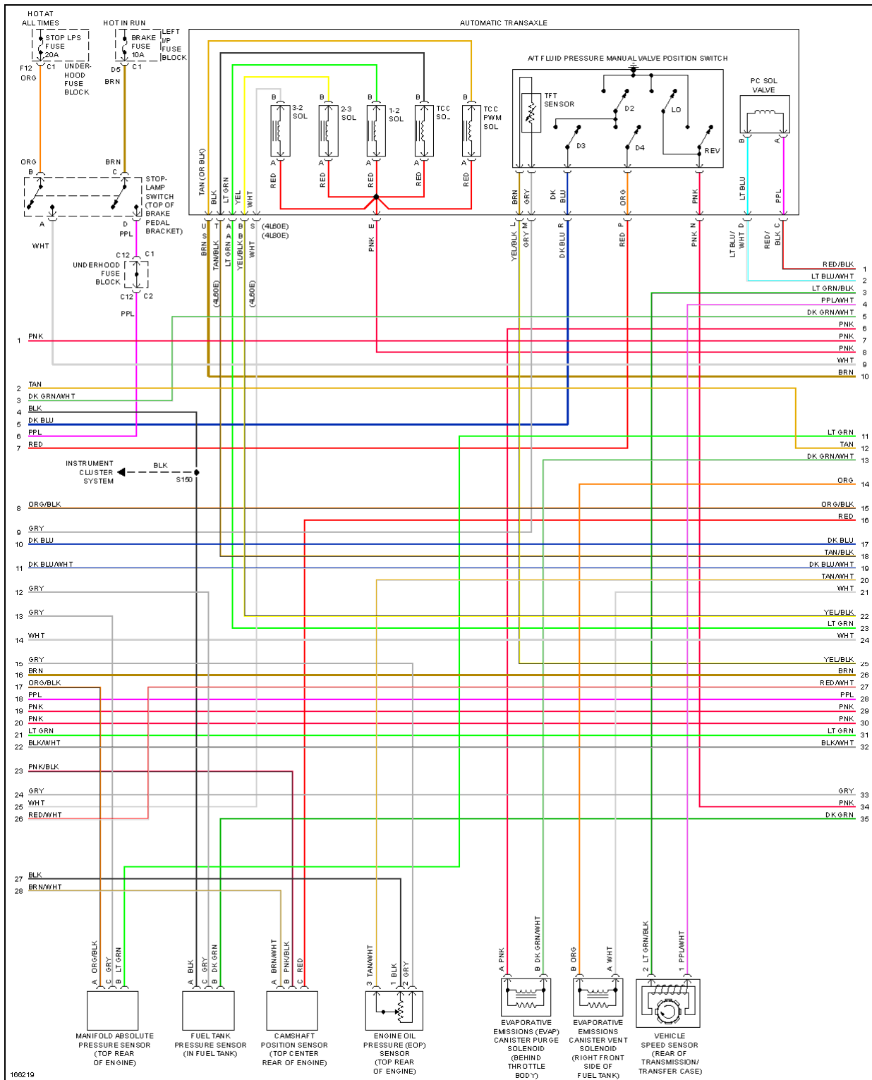
Fig. 25: 6.0L VIN N, Engine Performance Circuit (3 of 5)
