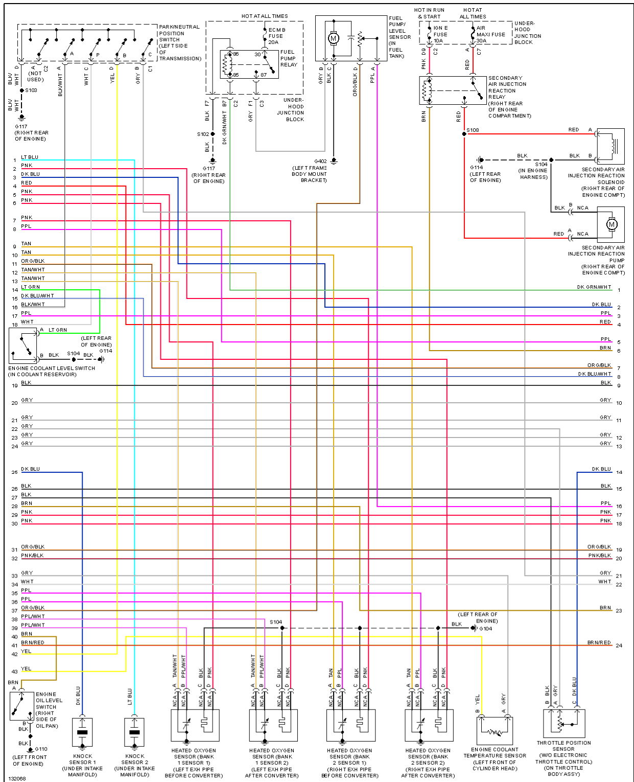
Fig. 34: 5.3L VIN T, Engine Performance Circuits, W/ Delphi HO2S (2 of 5)
