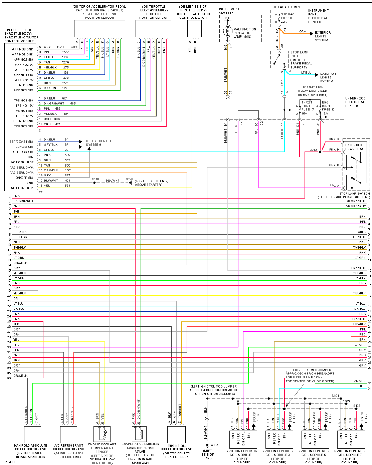
Fig. 16: 5.7L VIN G, Engine Performance Circuits (3 of 4)
