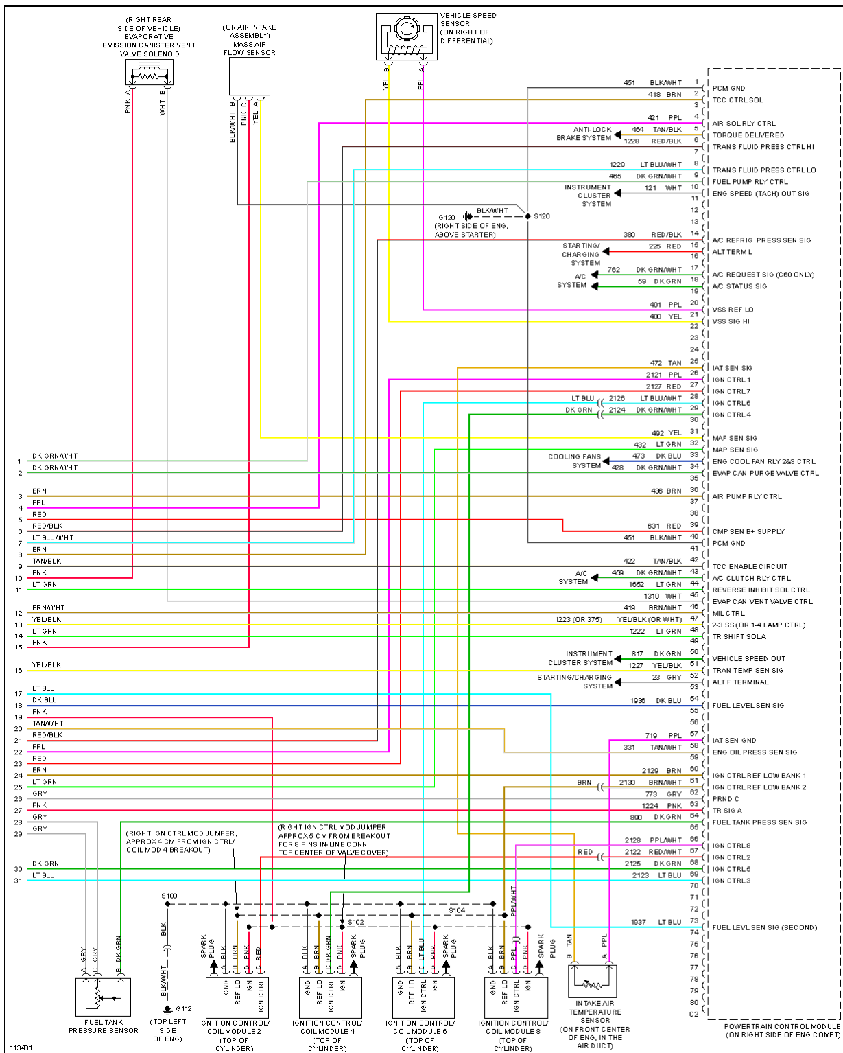
Fig. 17: 5.7L VIN G, Engine Performance Circuits (4 of 4)
