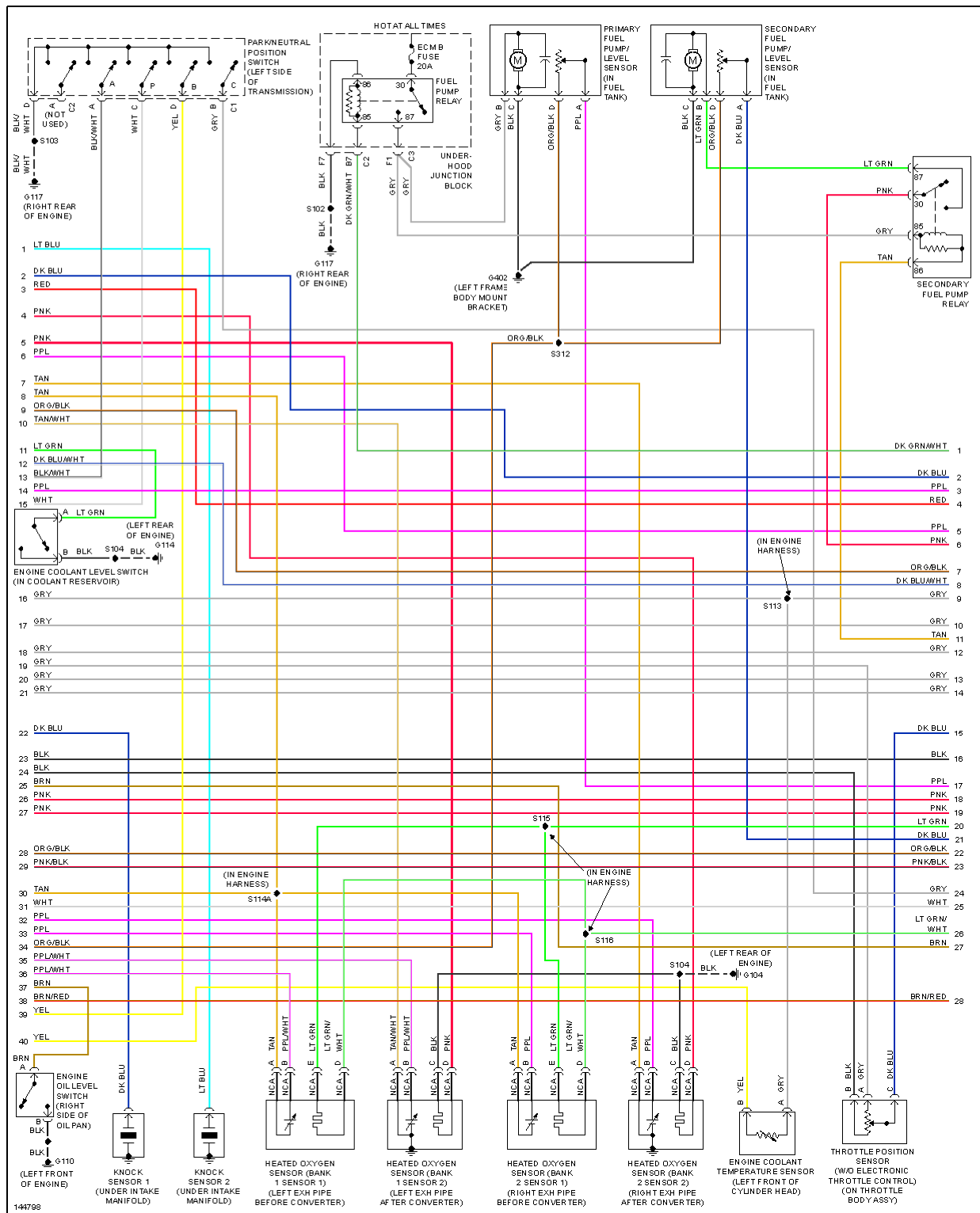
Fig. 17: 6.0L VIN U, Engine Performance Circuits (2 of 5)
