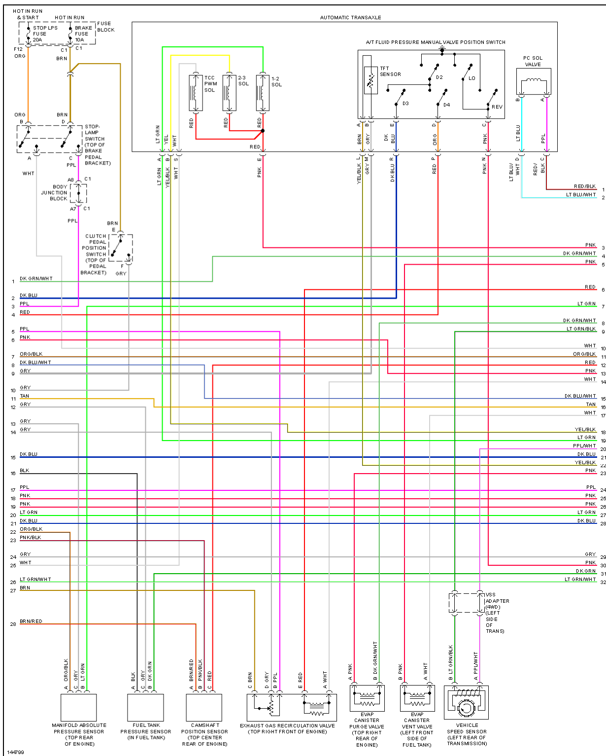
Fig. 18: 6.0L VIN U, Engine Performance Circuits (3 of 5)
