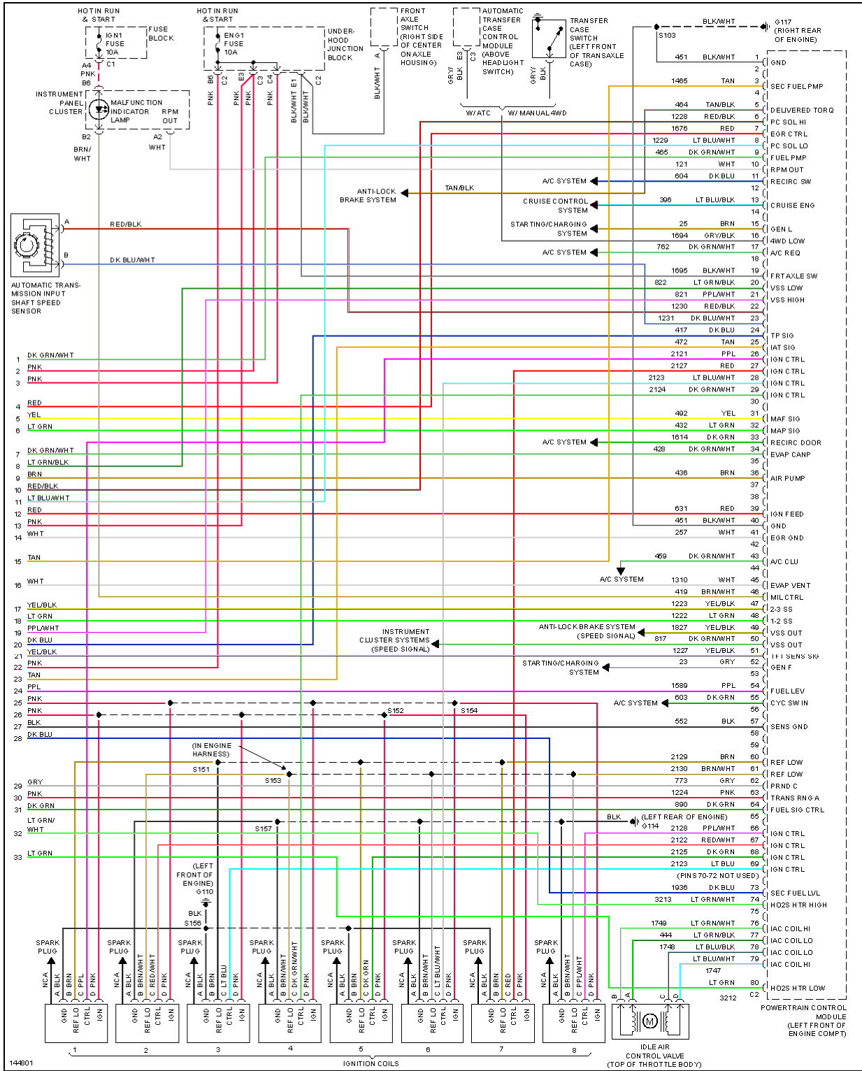
Fig. 20: 6.0L VIN U, Engine Performance Circuits (5 of 5)
