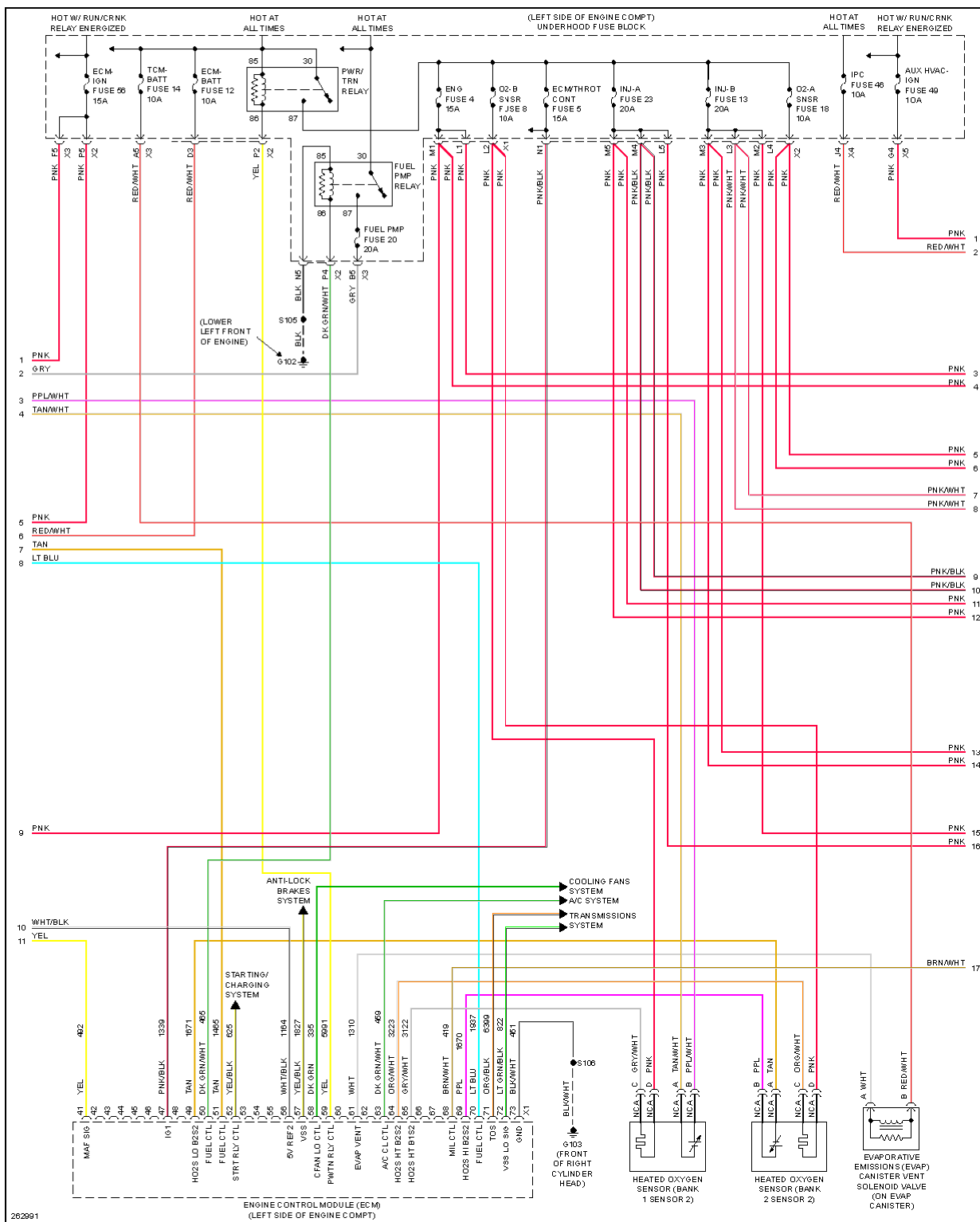
Fig. 26: 6.2L VIN 8, Engine Performance Circuit (2 of 5)
